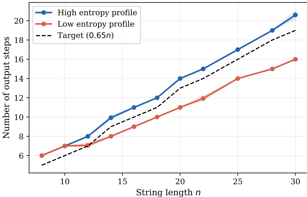
Step count scales linearly with string length
