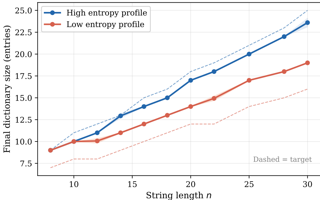
Dictionary growth scales with length; high entropy grows faster
