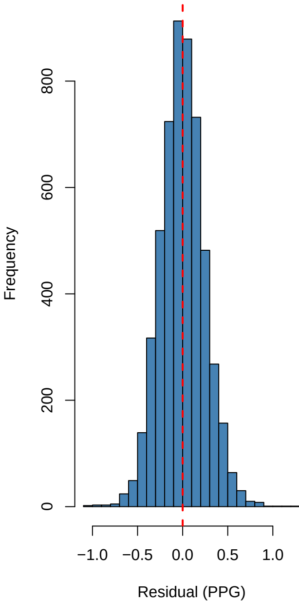
Residual distribution
