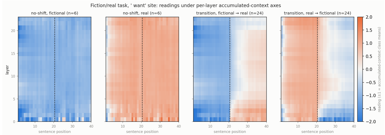
Figure 3: The same view for the fiction/real task: readings by layer and position, under axes refit per layer on accumulated no-shift contexts (class means at \pm 1 , so blue is the fictional side and red the real side). Left two panels: no-shift runs of each class, 6 runs each. Right two panels: transition runs in each direction, 24 each, with the shift after sentence 20. The dashed line marks sentence 20 in every panel. Every layer carries class signal, and no layer reads outside the range the two no-shift classes span.
