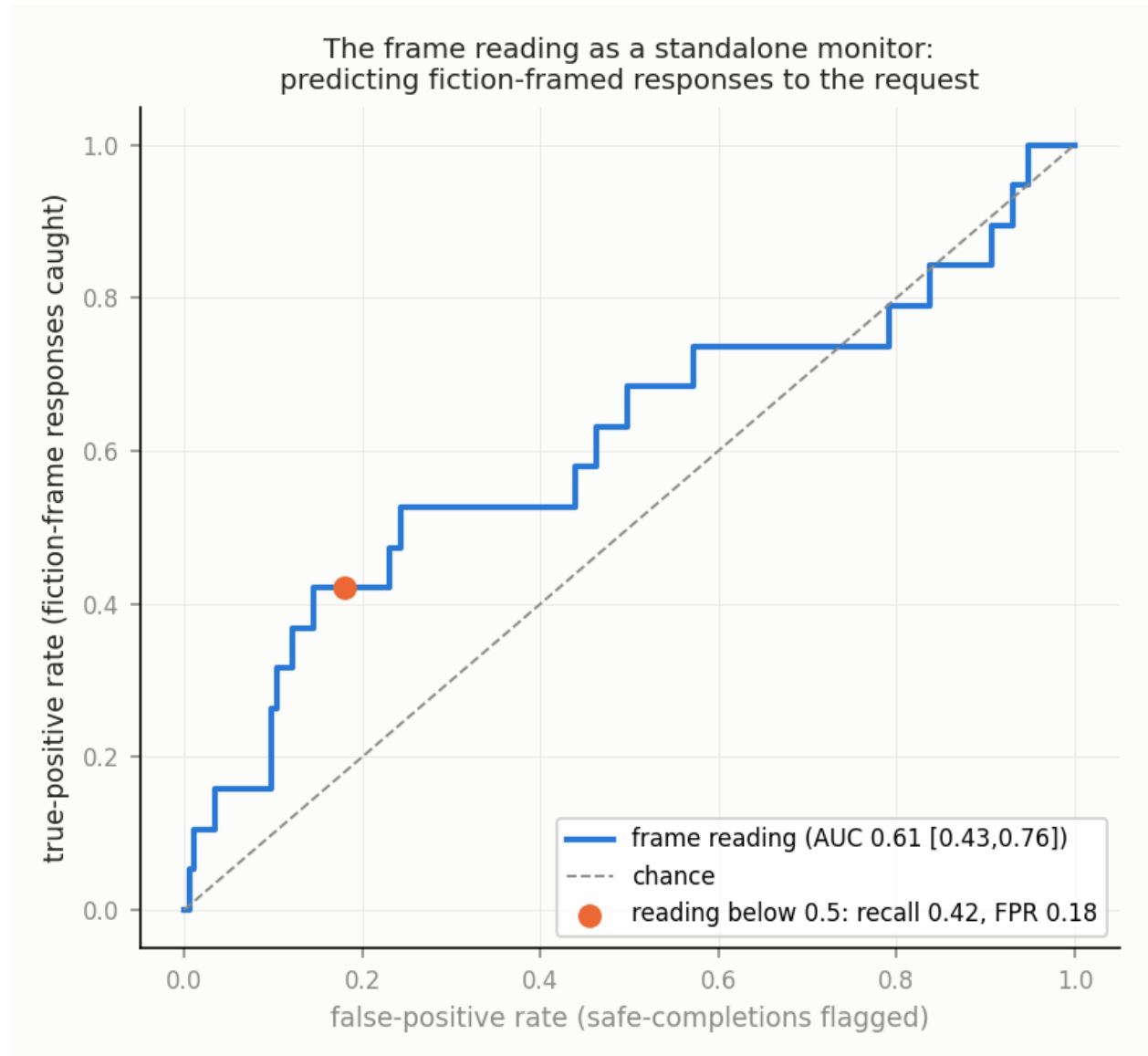
Figure 23: The frame reading as a standalone monitor, an exploratory check added after the analysis freeze. Receiver operating characteristic for predicting fiction-framed responses to the request (responses that take up the fictional frame rather than safe-completing) from the calibrated-site reading alone: the true-positive rate (fiction-framed responses caught) against the false-positive rate (safe-completions flagged). The AUC is 0.61 [0.43, 0.76], with a 95% interval clustered by scene family (§2.3), compatible with chance (dashed line). The marked point is one threshold, with its recall and false-positive rate.
