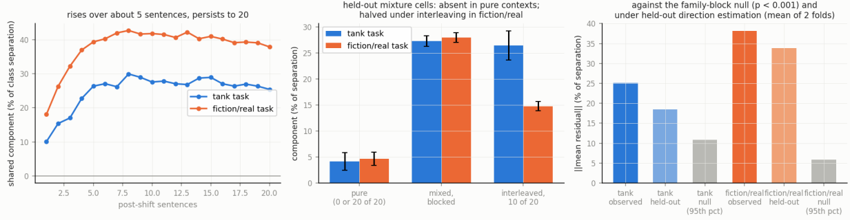
Figure 22: The mixed-context marker. Left: the mean displacement of transition states outside the no-shift principal-component subspace, projected on the shared direction and expressed as a percentage of the class separation, by post-shift sentence. It rises over about five sentences and persists to twenty. Middle: held-out mixture cells from the static sweeps. The marker is near zero in pure-class contexts (0 or 20 destination sentences of 20), near full strength in blocked mixtures, and, in the fiction/real task only, halved when the mixture is interleaved; error bars are one standard error over cells. Right: the observed mean displacement against the 95th percentile of a null built by resampling whole scene families ( p < 0.001 in both tasks), and its value under held-out direction estimation, the mean of two folds.
