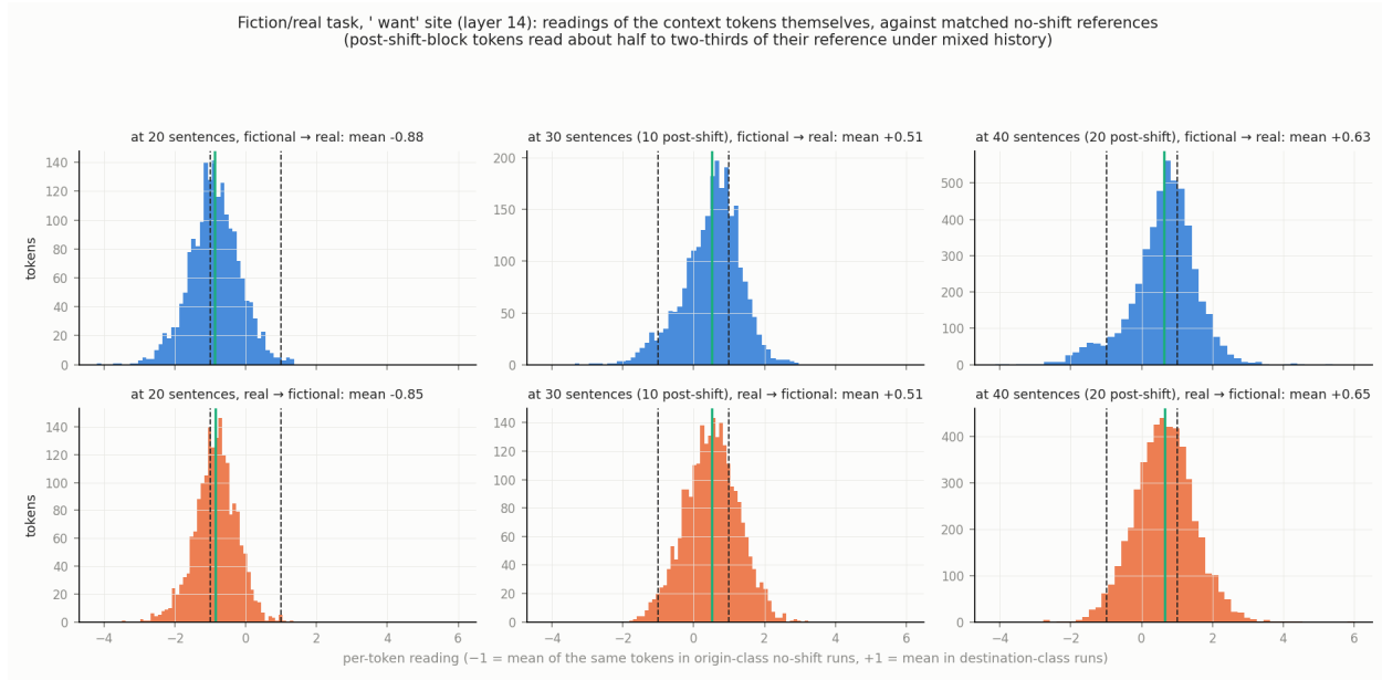
Figure 15: The same measurement in the fiction/real task (‘ want’ site, layer 14), which has a tighter instrument and no heavy tails. Top: fictional→real; bottom: real→fictional; panels at 20, 30, and 40 sentences. At 20 sentences the block reads near -1 , its origin-class baseline. The post-shift-block tokens read about half of the way to their no-shift reference at +1 at 30 sentences and about two-thirds at 40 (means in the panel titles).
