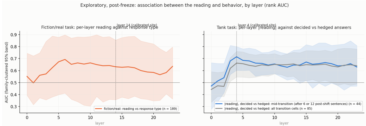
Figure 19: Exploratory, added after the analysis freeze: the association between the reading and behavior at every layer, as a rank AUC with family-clustered 95% bands. Left: the fiction/real task, reading against response type (189 completions). Right: the tank task, absolute reading against decided versus hedged answers, for mid-transition completions (44, at 6 and 12 post-shift sentences) and for all transition completions (85). Dotted lines mark the calibrated sites. The curves are roughly flat from mid-stack to the final layer in both tasks. The instrument is blunt: a band-level association with imbalanced outcomes.
