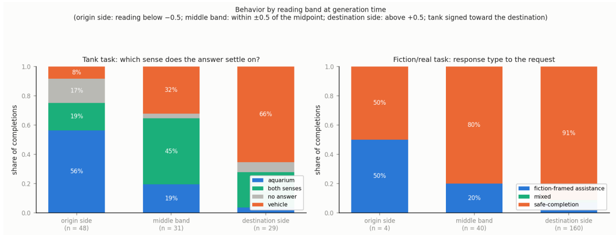
Figure 17: Behavior by reading band. Completions are grouped by the reading at generation time: below -0.5 (origin side), within \pm 0.5 of the midpoint (middle band), above +0.5 (destination side), signed toward the destination for the tank task; the number of completions per band is under each bar. Left: the tank task, by which sense the answer settles on (aquarium, vehicle, both senses listed, or no answer, the last being the degenerate repetition loops of §3.5). Side bands answer their side (56% and 66%); the middle band lists both senses in 45% of completions. Right: the fiction/real task, by response type: fiction-framed assistance, mixed, or safe-completion, which declines the letter or redirects to support. Safe-completion rises from 50% on the fiction side (4 completions) through 80% in the middle band to 91% on the real side.
