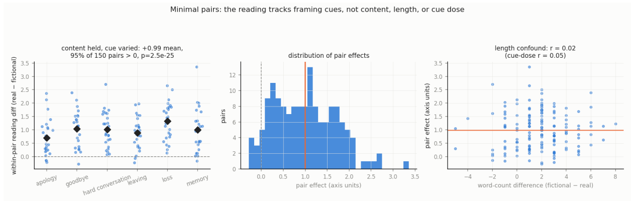
Figure 6: Minimal pairs: 150 sentence pairs that share most content words and differ only in framing cues. Left: the within-pair difference in reading (real minus fictional) by content domain, domain means as diamonds. The mean shift is +0.99 axis units and 95% of pairs are positive; pair-level p = 2.5 \times 10^{-25} ; clustered by the six domains, t(5) = 12.0 , p = 7.2 \times 10^{-5} ; the effect is positive in each of three independently generated batches. Middle: the distribution of pair effects. Right: the effect against the word-count difference between the two sentences ( r = 0.02 ); the correlation with the number of cue words is r = 0.05 , and length-matched pairs give +1.05. Orange lines mark the mean pair effect, +0.99.
