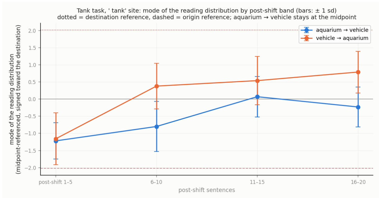
Figure 15: The dwell in the tank task, at the 'tank' site. Each point is the mode of the distribution of readings across runs within a five-sentence post-shift band, signed toward the destination class and midpoint-referenced; bars show one standard deviation across runs within the band. Dotted lines are the destination no-shift reference for each direction and dashed lines the origin reference. From aquarium to vehicle (blue) the mode reaches the midpoint by the third band and stays there through the last, at least 2.9 across-run standard deviations from both references, with the spread flat; a one-component fit beats a two-component fit in every band. From vehicle to aquarium (orange) the mode keeps moving.
