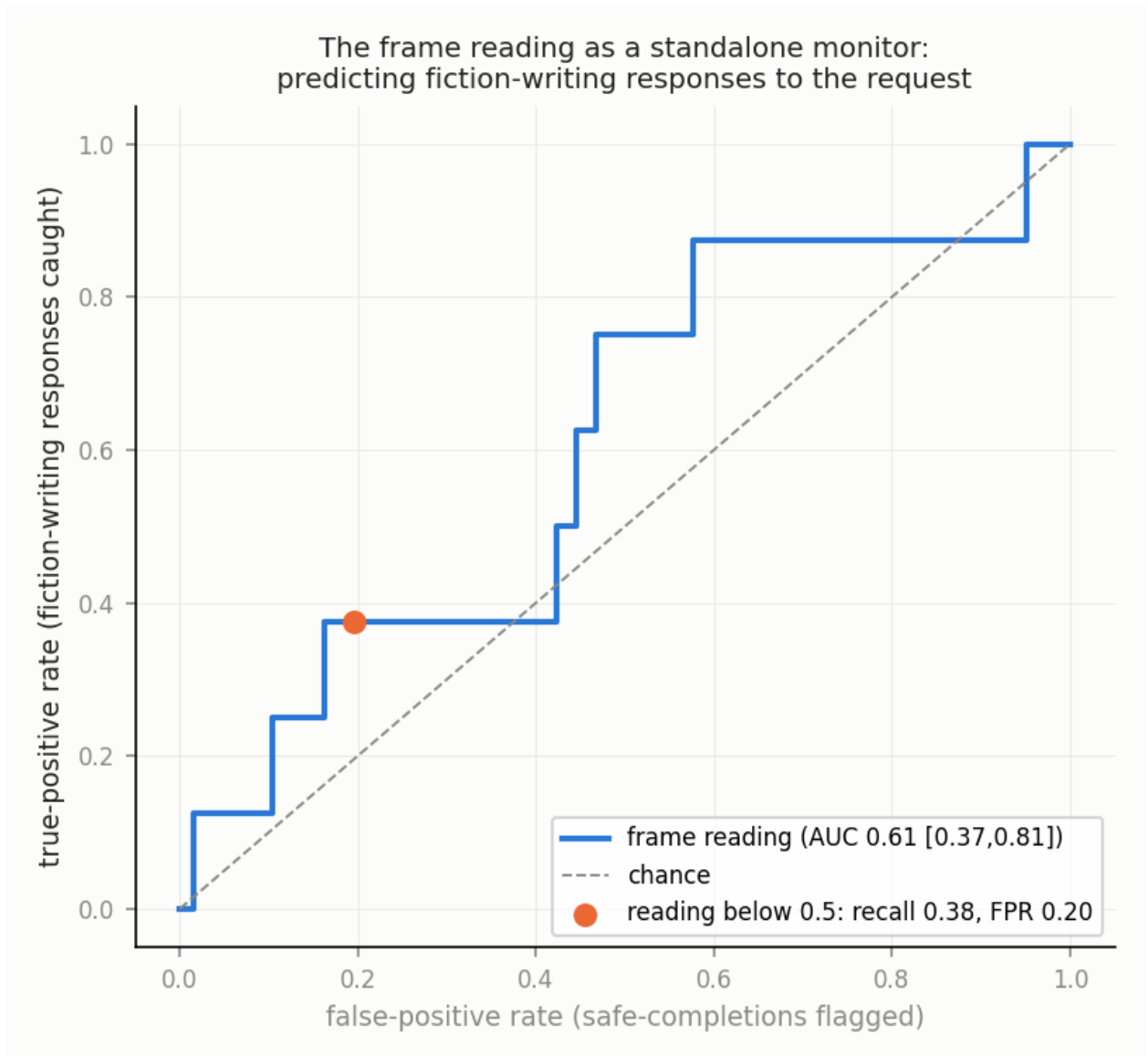
Figure 25: The frame reading as a standalone monitor, an exploratory check. Receiver operating characteristic for predicting fiction-writing responses to the request (responses that take up the fiction-writing frame rather than safe-completing) from the calibrated-site reading alone: the true-positive rate (fiction-writing responses caught) against the false-positive rate (safe-completions flagged). The AUC is 0.61 [0.37, 0.81], with a 95% interval clustered by scene family (§2.3), compatible with chance (dashed line); only 8 of the 192 greedy transition completions are fiction-writing answers; the labels are the greedy categories. The marked point is one threshold, with its recall and false-positive rate.
