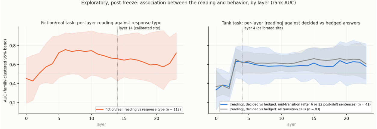
Figure 21: Exploratory: the association between the reading and behavior at every layer, as a rank AUC with family-clustered 95% bands. Left: the fiction/real task, reading against response type (112 delivered transition answers). Right: the tank task, absolute reading against decided versus hedged answers, for mid-transition completions (41 delivered, at 6 and 12 post-shift sentences) and for all transition completions (83 delivered). Dotted lines mark the calibrated sites. The curves are roughly flat from mid-stack to the final layer in both tasks. The instrument is blunt: a band-level association with imbalanced outcomes.
