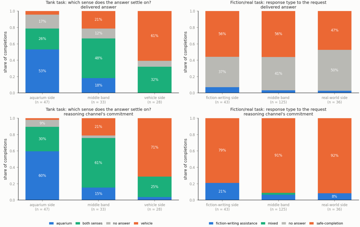
Figure 18: Greedy behavior by reading band, read two ways. Completions are grouped by the reading at generation time, referenced to the position-matched midpoint of the two no-shift classes and cut at \pm 0.5 axis units: the aquarium side and the fiction-writing side below, the middle within, the vehicle side and the real-world side above. The number of contexts per band is under each bar. Top row: the delivered answer, with gray the share of outputs that never delivered one under greedy decoding. Bottom row: what the reasoning channel committed to in the same contexts, which every context has. Left: the tank task, by which sense the answer settles on. The side bands answer their own side (64% and 65% of delivered answers) and the middle band lists both senses in 55% of delivered answers. Right: the fiction/real task, by response type. Delivered answers safe-complete in 89% of the fiction-writing side, 95% of the middle band, and 94% of the real-world side; the reasoning channel commits to a safe completion in 79%, 91%, and 92% of the same bands. The gap between the rows is the loops, whose rate is higher on reasoning that had committed to fiction-writing assistance (15 of 23 against 70 of 181). Completions decoded greedily with a 2,048-token cap (§2.5); the sampled regime is in the next figure.
