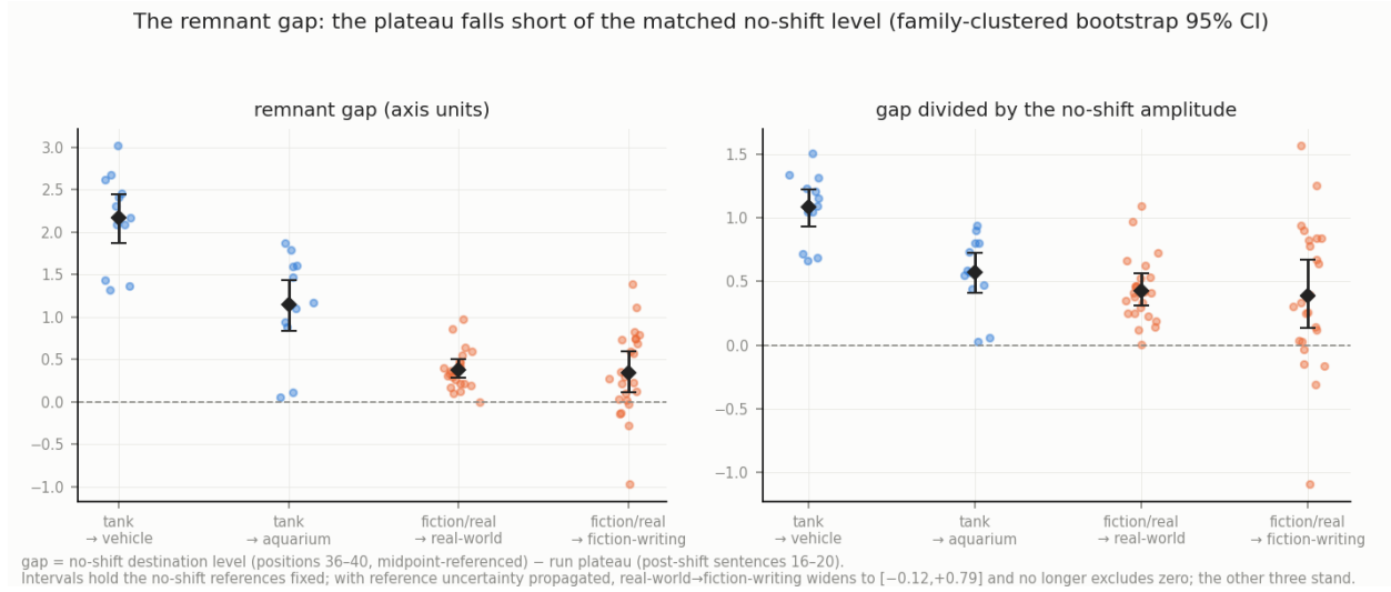
Figure 9: The remnant gap, run by run. Each dot is one transition run: the no-shift reference level minus the run’s plateau, both over positions 36–40 and both measured from the midpoint. Left, in axis units; right, divided by the no-shift amplitude, which is 2.0 in the tank task and 0.9 in fiction/real; even after this division the task with the wider endpoint separation shows the larger gaps. Each dot is one run: 12 per direction in the tank task and 24 in fiction/real. Diamonds are means with family-clustered bootstrap 95% intervals, holding the no-shift references fixed. With the references also resampled, three intervals still exclude zero and real-world→fiction-writing widens to [-0.12, +0.79] (Table 2). Blue: the tank task, toward vehicle and toward aquarium; orange: the fiction/real task, toward real-world and toward fiction-writing.
