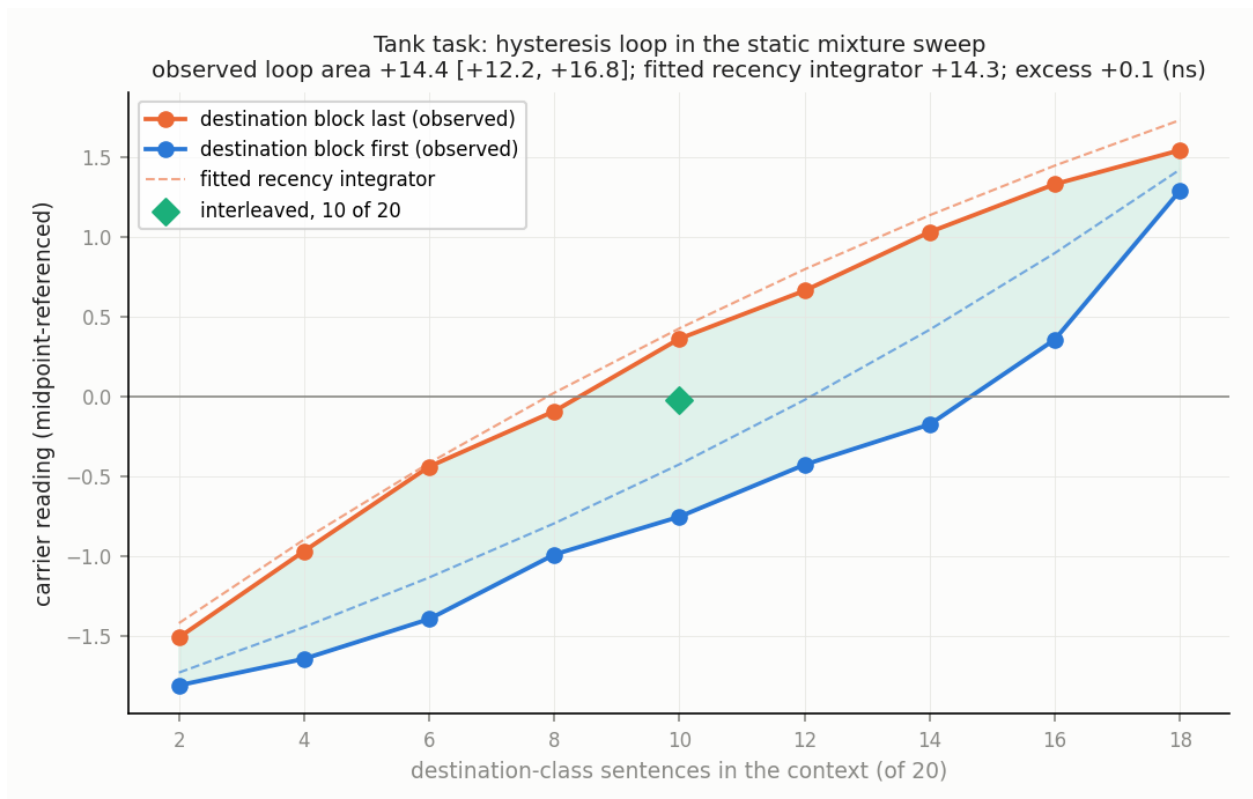
Figure 22: Hysteresis in the tank task. Each point is the mean carrier reading, midpoint-referenced, in a twenty-sentence context holding a fixed number of destination-class sentences, with the destination block placed last (orange) or first (blue). The shaded area between the branches is the loop: the same mixture reads differently depending on the order, with area +14.4 [12.2, 16.8]. Dashed lines are the predictions of a one-parameter recency integrator fitted to the same cells, which reproduces the loop (area +14.3); the excess, +0.1, is indistinguishable from zero. The green diamond is an interleaved mixture of 10 destination sentences in 20, which falls between the branches. The fiction/real sweep (Appendix C) gives +10.5 [7.5, 13.3] observed against +11.1 fitted (Table 6).
