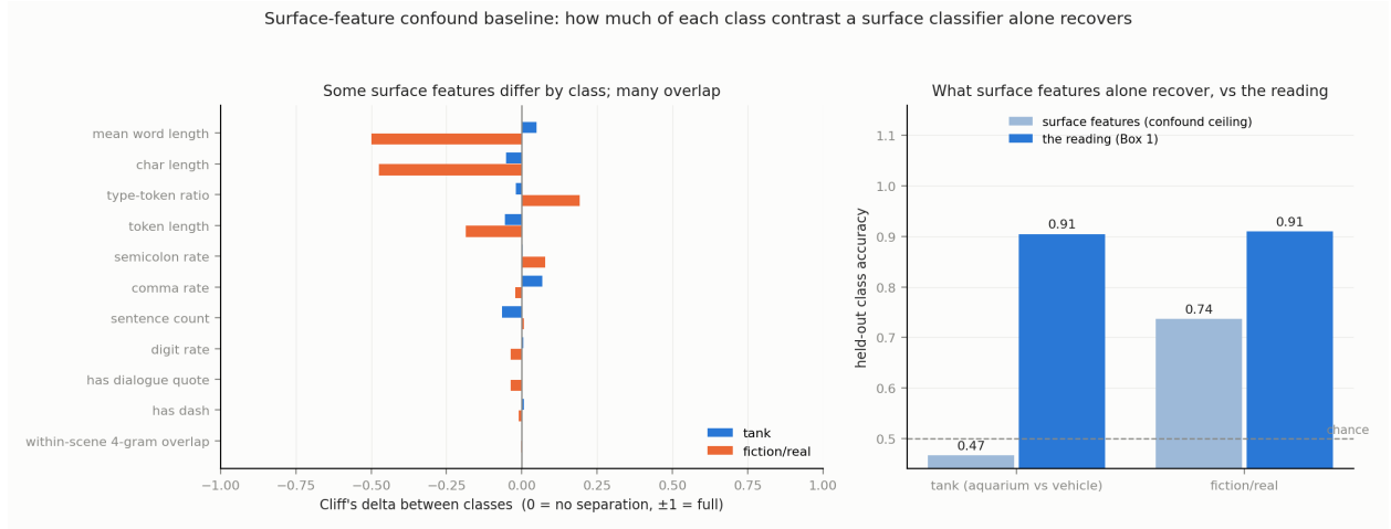
Figure 8: The surface-feature confound baseline of §3.1. Deterministic surface features only — token and character length, sentence count, type-token ratio, comma/semicolon/dialogue/digit rates, opener class, and within-scene 4-gram overlap — computed from the sentence text with no access to the residual stream. Left: Cliff’s delta between the two classes per feature (0 = full overlap, \pm 1 = full separation), for each task; most features overlap, and the fiction/real classes differ mainly in length and type-token ratio. Right: how much of each class contrast a standardized logistic classifier recovers from these features alone, validated leave-one-scene-pair-out (the confound ceiling), beside the reading’s own held-out accuracy (Box 1). On the tank task the surface classifier is at chance, balanced accuracy 0.47, while the reading reaches 0.905; on the fiction/real task surface features carry real signal, 0.74, as the framing is itself cued by surface form, yet the reading separates the classes better, at 0.910.
