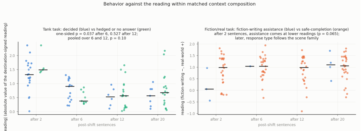
Figure 20: Greedy behavior against the reading at matched context composition, that is, among completions generated after the same number of post-shift sentences under greedy decoding. Left: the tank task. Each dot is the absolute value of one completion’s reading, taken after signing the reading toward the destination class, split by whether the answer settled on one sense (blue) or listed both or gave no answer (green); bars are medians. After 6 post-shift sentences decided answers come from runs with more extreme readings (medians 0.90 against 0.38, one-sided p = 0.037 ); after 12 they do not (0.53 against 0.56), and the pooled test over 6 and 12 gives 0.67 against 0.55 ( p = 0.10 ). Right: the fiction/real task, reading by response type, fiction-writing assistance (blue) or safe-completion (orange); outputs that delivered no answer are excluded. After 2 post-shift sentences assistance comes at lower readings (medians +0.06 against +0.99, 3 answers against 26, p = 0.065 ); at later counts the reading does not separate the types.
