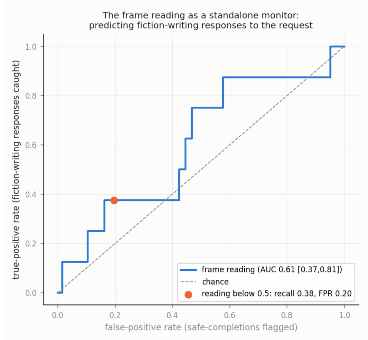
Figure 24: The frame reading as a standalone monitor, an exploratory check. Receiver operating characteristic for predicting fiction-writing responses to the request (responses that take up the fiction-writing frame rather than safe-completing) from the calibrated-site reading alone: the true-positive rate (fiction-writing responses caught) against the false-positive rate (safe-completions flagged). The AUC is 0.61 [0.37, 0.81], with a 95% interval clustered by scene family (§2.3), compatible with chance (dashed line); only 8 of the 192 greedy transition completions are fiction-writing answers; the labels are the greedy categories. The marked point is one threshold, with its recall and false-positive rate.
