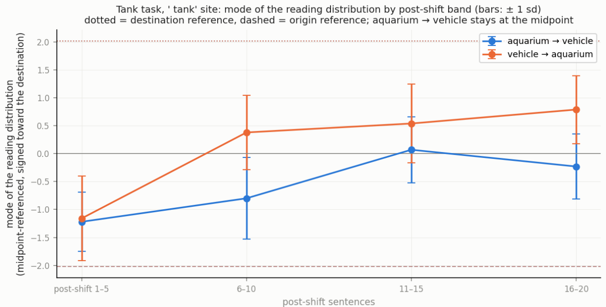
Figure 16: The dwell in the tank task, at the ‘tank’ site. Each point is the mode of the distribution of readings across runs within a five-sentence post-shift band, signed toward the destination class and midpoint-referenced; bars show one standard deviation across runs within the band. Dotted lines are the destination no-shift reference for each direction and dashed lines the origin reference. From aquarium to vehicle (blue) the mode reaches the midpoint by the third band and stays there through the last, at least 2.9 across-run standard deviations from both references, with the spread flat; a one-component fit beats a two-component fit in every band. From vehicle to aquarium (orange) the mode keeps moving.
