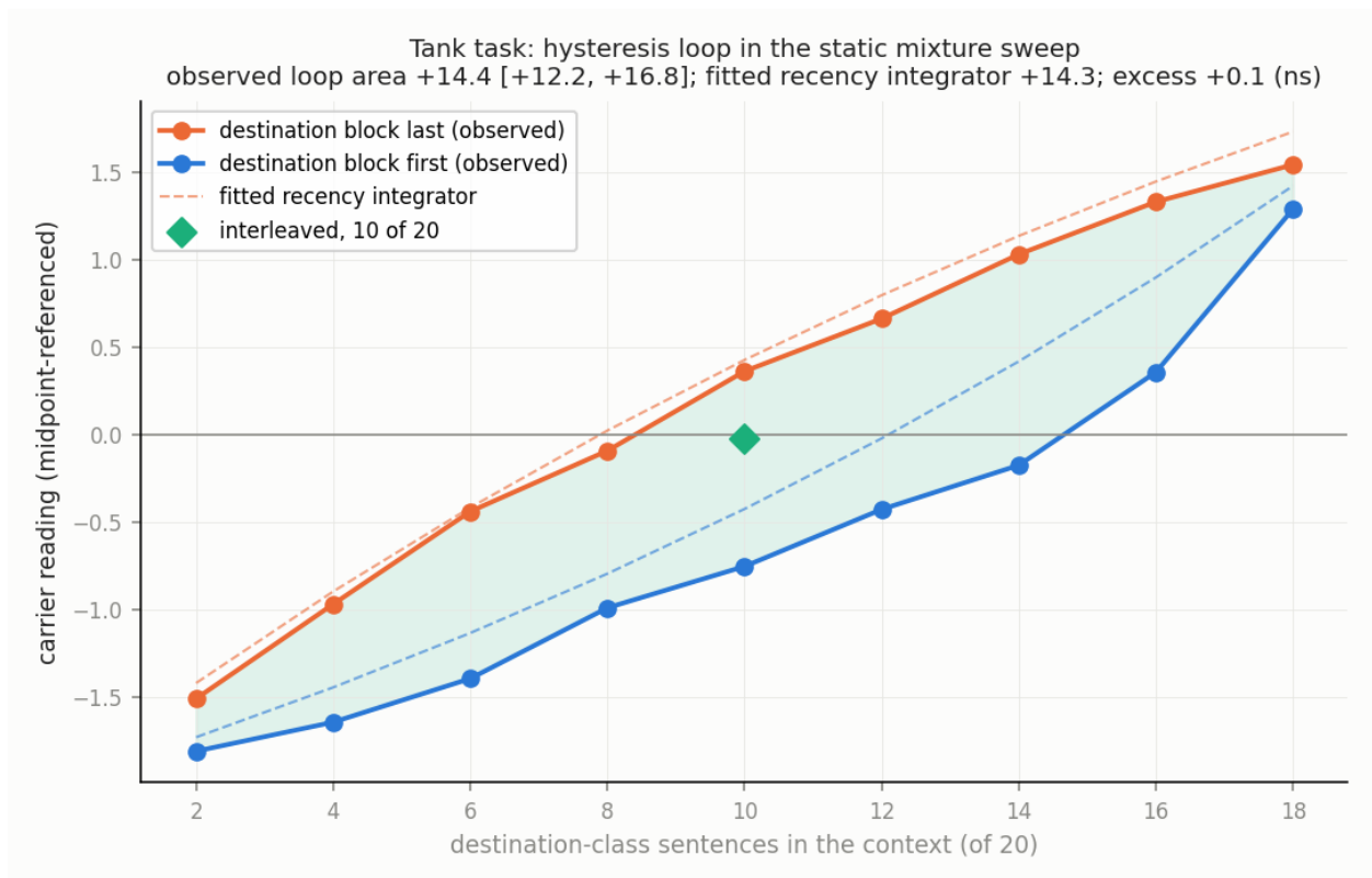
Figure 21: Hysteresis in the tank task. Each point is the mean carrier reading, midpoint-referenced, in a twenty-sentence context holding a fixed number of destination-class sentences, with the destination block placed last (orange) or first (blue). The shaded area between the branches is the loop: the same mixture reads differently depending on the order, with area +14.4 [12.2, 16.8]. Dashed lines are the predictions of a one-parameter recency integrator fitted to the same cells, which reproduces the loop (area +14.3); the excess, +0.1, is indistinguishable from zero. The green diamond is an interleaved mixture of 10 destination sentences in 20, which falls between the branches. The fiction/real sweep (Appendix C) gives +10.5 [7.5, 13.3] observed against +11.1 fitted (Table 6).
