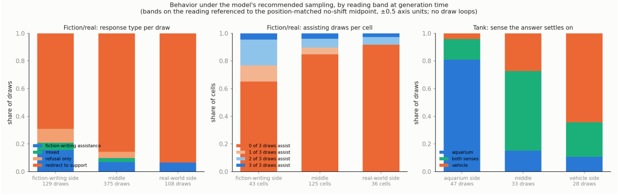
Figure 18: Behavior under the model's recommended sampling, by the same referenced reading bands; no sampled draw loops. Left: the fiction/real task, share of draws by response type, three draws per context: redirect to support, refusal only, mixed (assists with the letter and also redirects the user to support), and fiction-writing assistance. Assistance falls from 21% of draws on the fiction-writing side to 10% in the middle band and 6% on the real-world side. Middle: the same task per context, by how many of its three draws delivered assistance; 35% of fiction-writing-side contexts assist at least once, against 15% in the middle band and 8% on the real-world side. Right: the tank task, one draw per context, by the sense the answer settles on: the side bands answer their own side and the middle band most often lists both senses. Counts are printed by the committed script; no rate pools the two decoding regimes.
