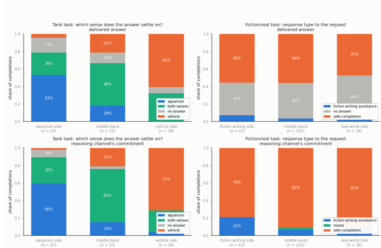
Behavior by reading band at generation time: the delivered answer (top) and the reasoning channel's commitment (bottom) (bands on the reading referenced to the position-matched no-shift midpoint: below -0.5 , within \pm 0.5 , above +0.5 axis units; negative is the aquarium side and the fiction-writing side)
