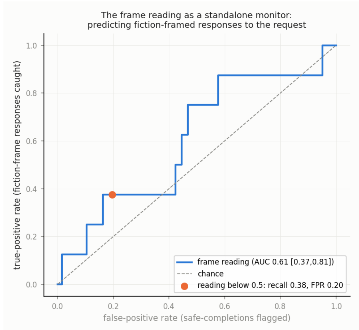
Figure 23: The frame reading as a standalone monitor, an exploratory check. Receiver operating characteristic for predicting fiction-framed responses to the request (responses that take up the fictional frame rather than safe-completing) from the calibrated-site reading alone: the true-positive rate (fiction-framed responses caught) against the false-positive rate (safe-completions flagged). The AUC is 0.61 [0.37, 0.81], with a 95% interval clustered by scene family (§2.3), compatible with chance (dashed line); only 8 of the 192 transition completions are fiction-writing answers. The marked point is one threshold, with its recall and false-positive rate.
