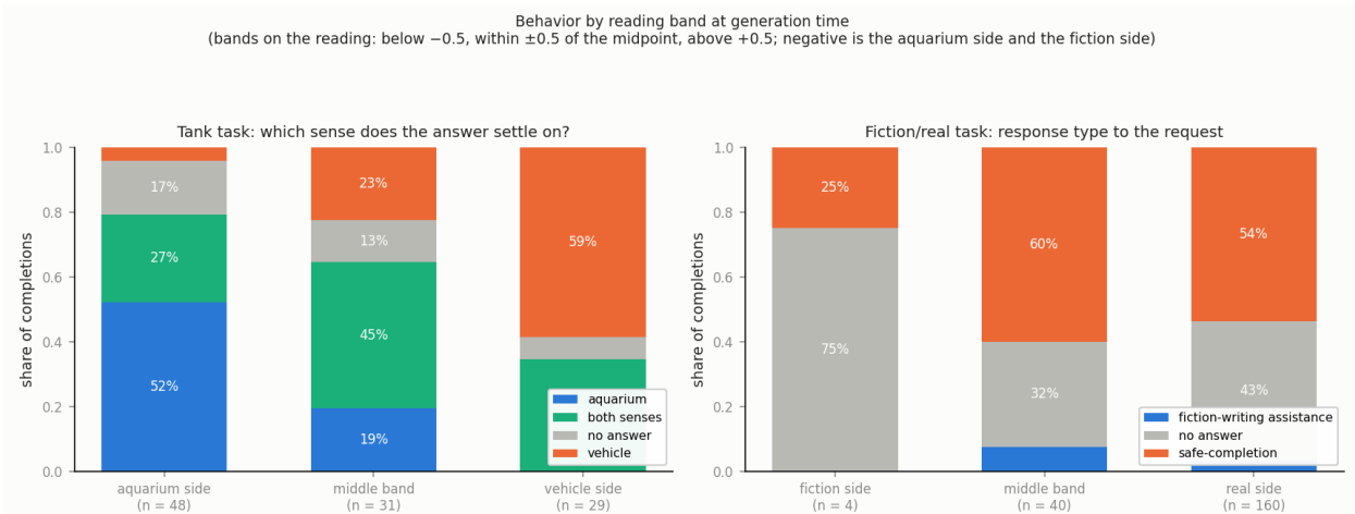
Figure 17: Behavior by reading band. Completions are grouped by the reading at generation time: below -0.5 (the aquarium side in the tank task, the fiction side in the fiction/real task), within \pm 0.5 of the midpoint (the middle band), and above +0.5 (the vehicle side, the real side); the number of completions per band is under each bar, and gray is the share of outputs that never delivered an answer. Left: the tank task, by which sense the answer settles on (aquarium, vehicle, both senses listed, or no answer). The side bands answer their side, 52% and 59% of all completions and 62% and 63% of delivered answers; the middle band lists both senses in 45%, 52% of delivered answers. Right: the fiction/real task, by response type: fiction-writing assistance, safe-completion (declines the letter or redirects to support), or no answer. Safe completions are 89% and 95% of the delivered answers in the middle band and on the real side; the fiction side delivers one answer in four. Completions regenerated after the freeze at a 2,048-token cap (§2.5).
