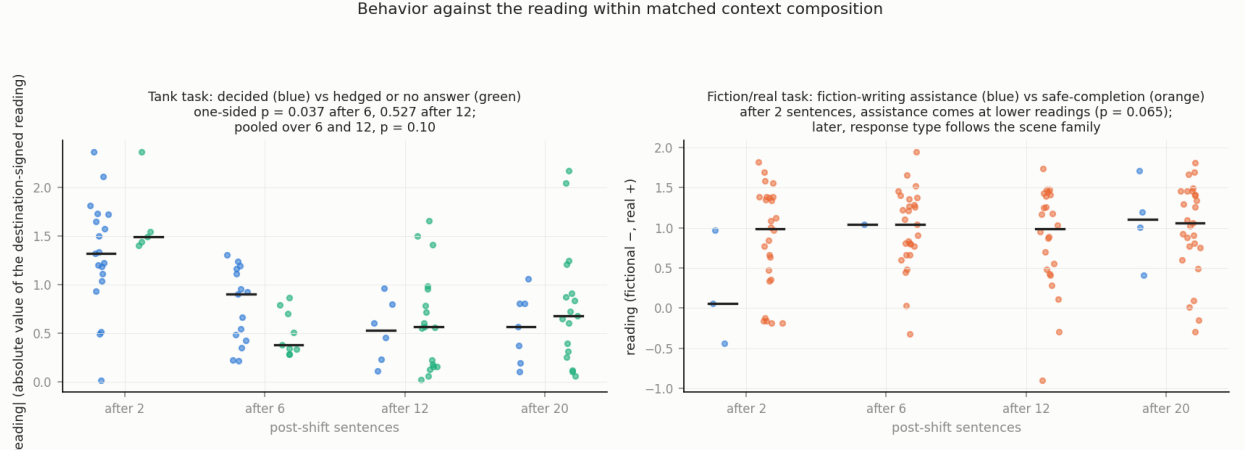
Figure 18: Behavior against the reading at matched context composition, that is, among completions generated after the same number of post-shift sentences, on the regenerated completions (§2.5). Left: the tank task. Each dot is the absolute value of one completion’s reading, taken after signing the reading toward the destination class, split by whether the answer settled on one sense (blue) or listed both or gave no answer (green); bars are medians. After 6 post-shift sentences decided answers come from runs with more extreme readings (medians 0.90 against 0.38, one-sided p = 0.037 ); after 12 they do not (0.53 against 0.56), and the pooled test over 6 and 12, pre-stated before the regenerated answers were read, gives 0.67 against 0.55 ( p = 0.10 ). Right: the fiction/real task, reading by response type, fiction-writing assistance (blue) or safe-completion (orange); outputs that delivered no answer are excluded. After 2 post-shift sentences assistance comes at lower readings (medians +0.06 against +0.99, 3 answers against 26, p = 0.065 ); at later counts the reading does not separate the types.
