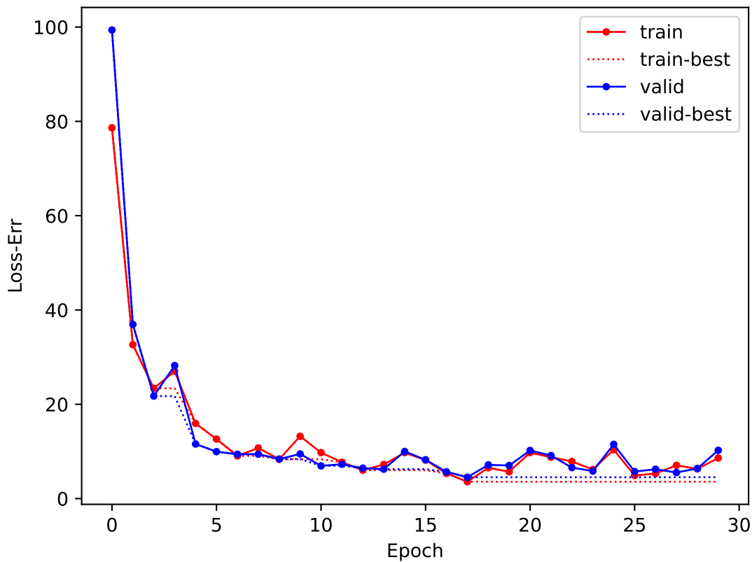
Loss-Err
