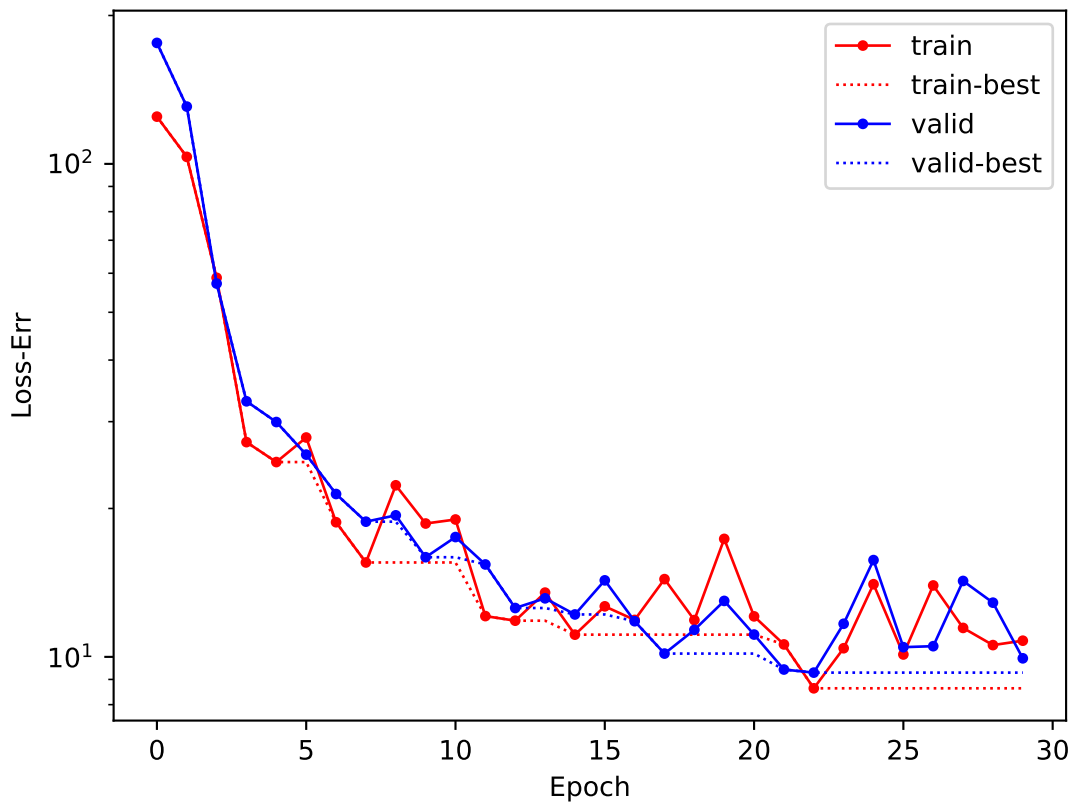
Loss-Err
