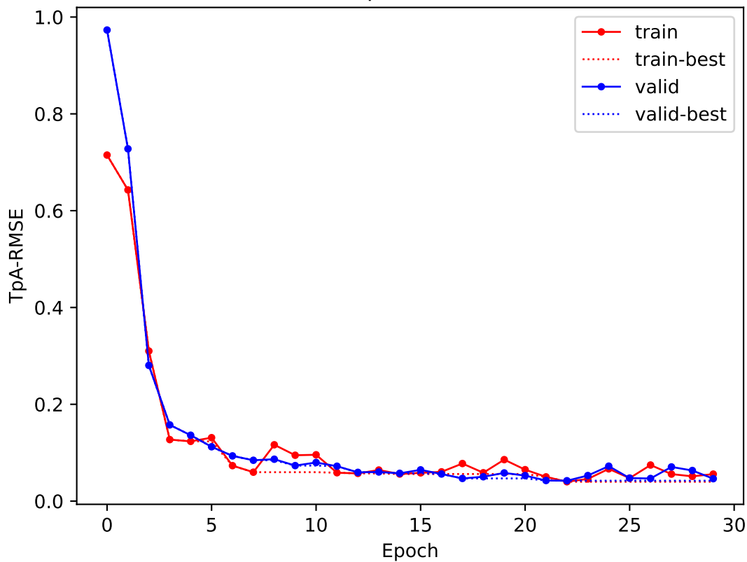
TpA-RMSE
