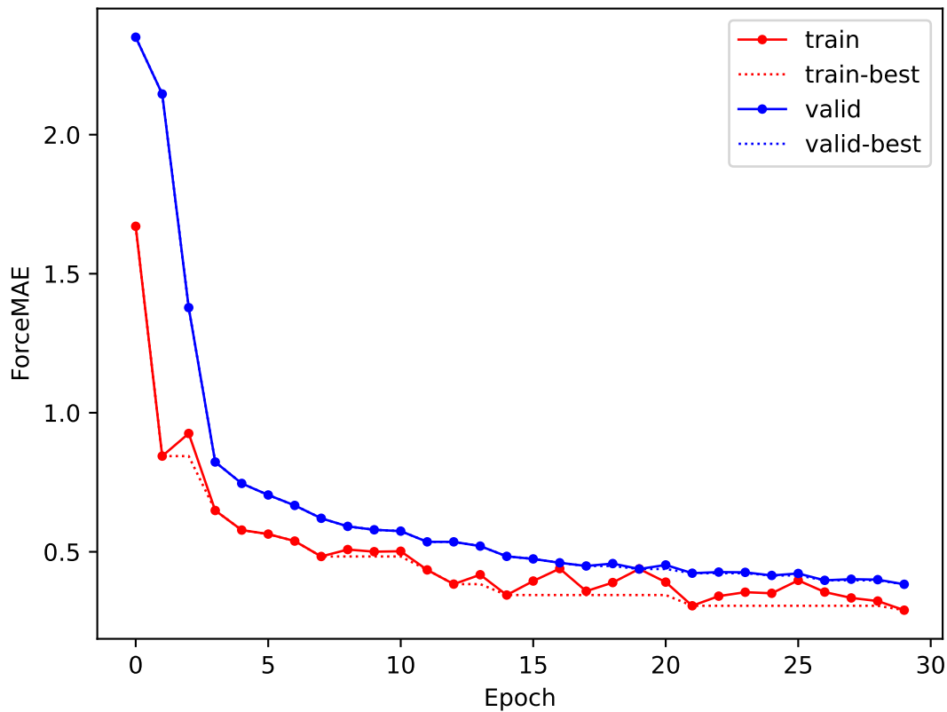
ForceMAE
