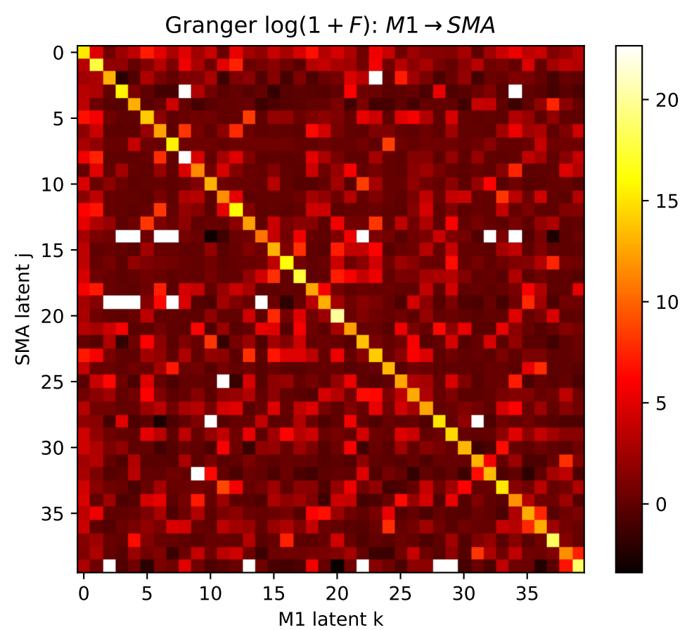
Latent-level interaction graph (lag=3 time steps)
