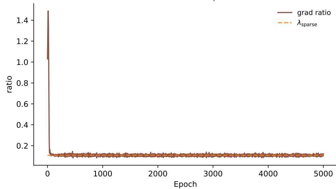
Grad ratio vs. \lambda_{\text{sparse}}
