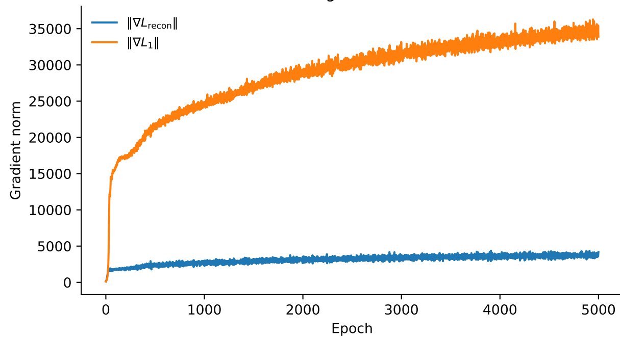
Encoder gradient norms
