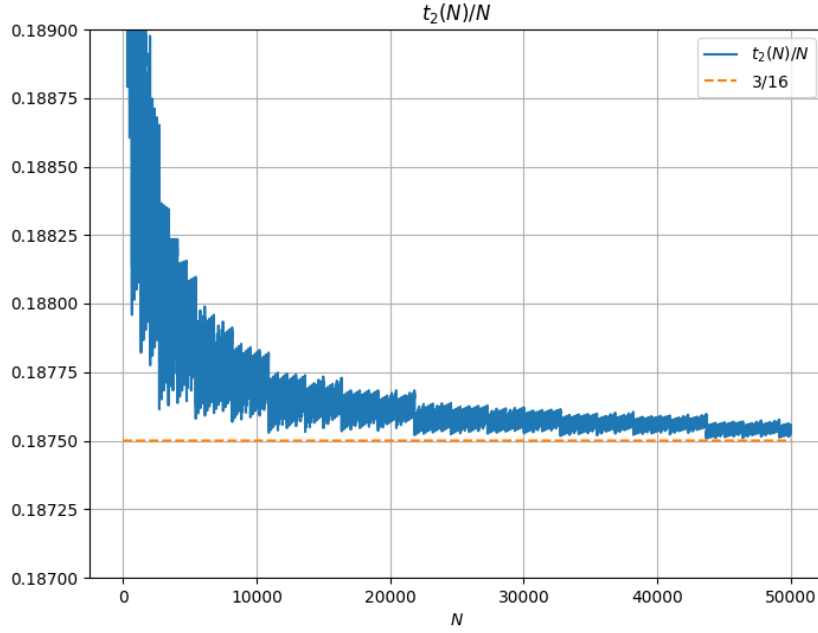
FIGURE 14. The function t_2(N)/N was computed exactly in [?], and converges quickly to 3/16 .
