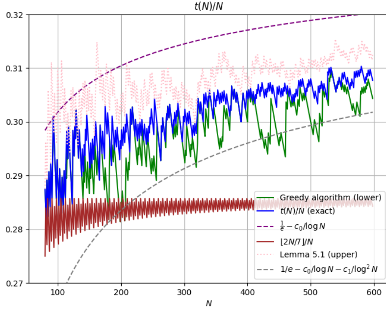
FIGURE 11. An enlarged version of ??, displaying the lower bound from the greedy algorithm and the upper bound from ?. The linear programming upper bound and floor+residual bounds are exact in this region, except for N = 155 in which the upper bound is off by one.
