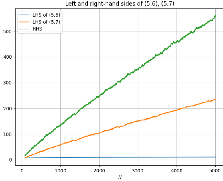
FIGURE 13. A plot of the left and right sides of (??), (??) for 80 \leq N < 5000 .
