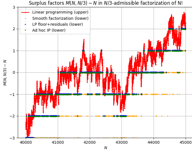
FIGURE 8. Bounds on M(N, N/3) - N for 4 \times 10^4 \leq N \leq 4.5 \times 10^4 . The linear programming upper bound (red) can be rounded down to the nearest integer, as per (??). In this range, at least one of the integer programming (green, implemented in an ad hoc fashion) and the floor+residuals (blue) methods turn out to match this bound exactly, with the smooth factorization method (orange) not far behind.
