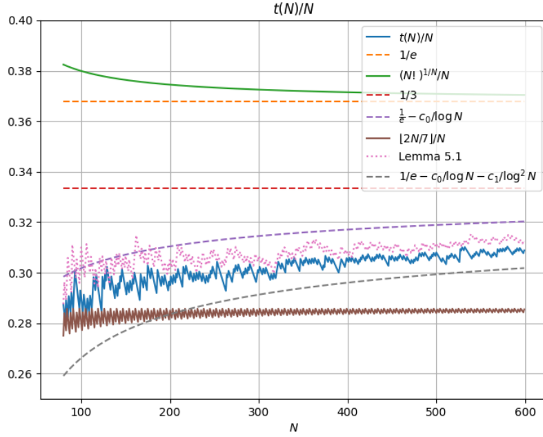
FIGURE 2. A continuation of ?? to the region 80 \leq N \leq 599 .
