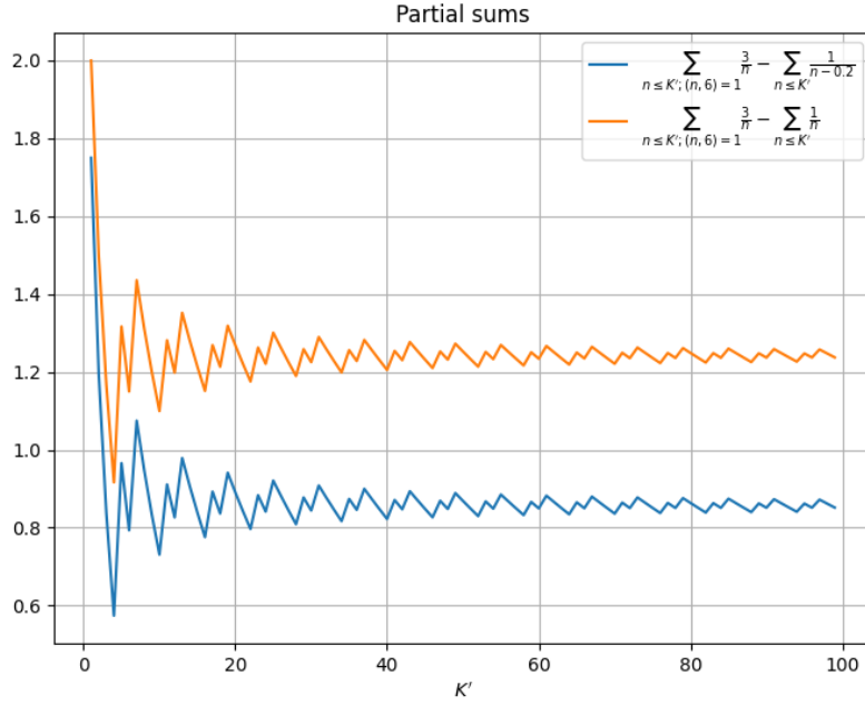
FIGURE 18. A plot of (??), (??).
