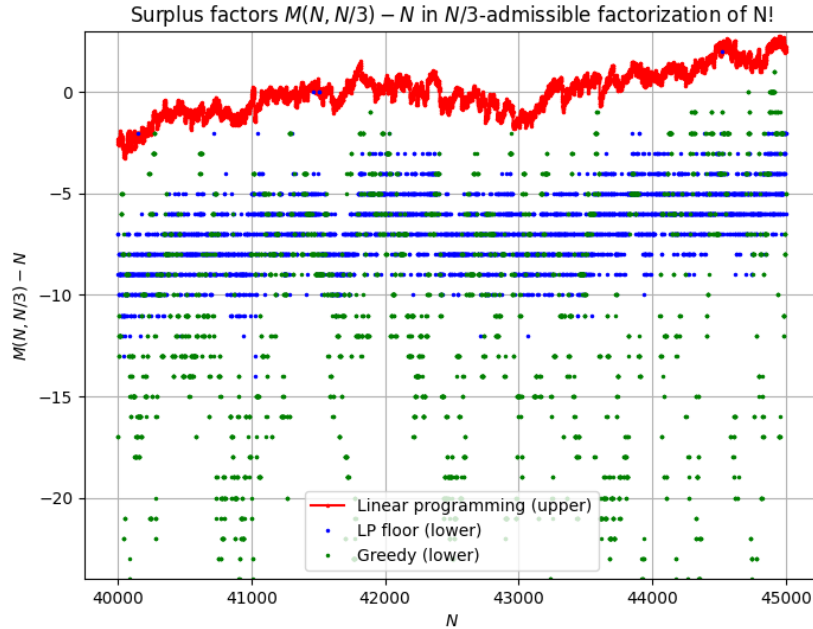
FIGURE 9. Two weaker lower bounds on M(N, N/3) - N for 4 \times 10^4 \leq N \leq 4.5 \times 10^4 beyond those depicted in ??: the floor of a linear programming method (blue) without gathering residuals, and the greedy method (green), which performs erratically but usually gives worse bounds than any of the other methods in this range.
