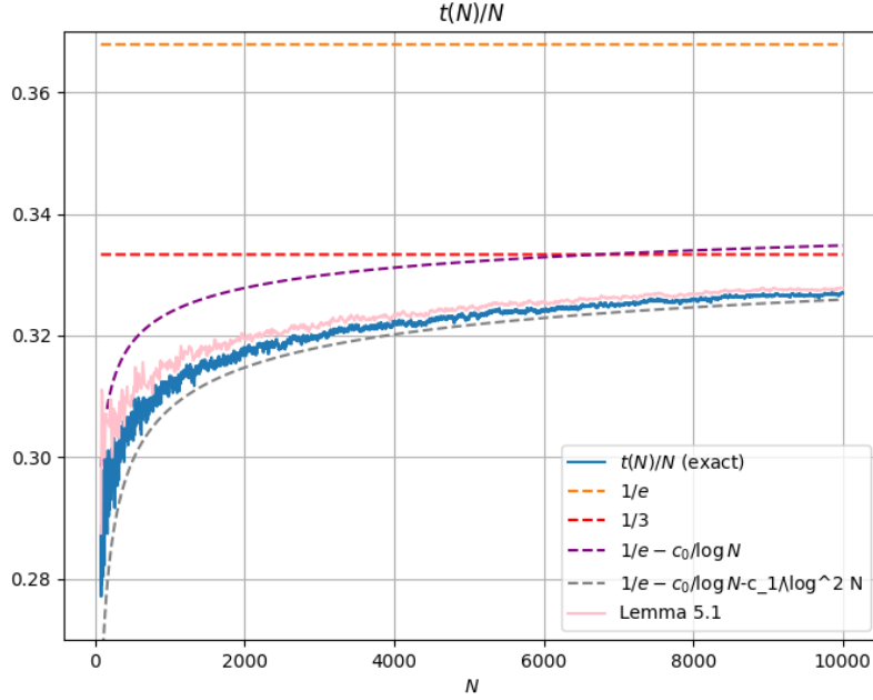
FIGURE 6. Exact values of t(N)/N for 80 \leq N \leq 10^4 , obtained via integer programming. The upper bound from ?? is surprisingly sharp, as is the refined asymptotic 1/e - c_0/\log N - c_1/\log^2 N , though the cruder asymptotics 1/e or 1/e - c_0/\log N are significantly poorer approximations.
