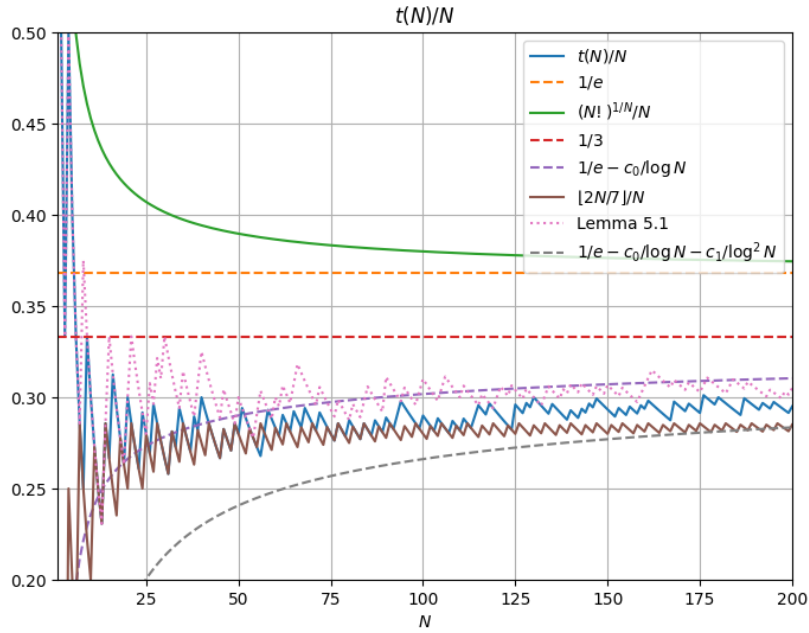
FIGURE 1. The function t(N)/N (blue) for N \leq 200 , using the data from OEIS A034258, as well as the trivial upper bound (N!)^{1/N}/N (green), the improved upper bound from ?? (pink), which is asymptotic to ?? (purple), and the function [2N/7]/N (brown), which we show to be a lower bound for N \neq 56 . ??(iv) implies that t(N)/N is asymptotic to ?? (purple), which in turn converges to 1/e (orange), although we believe that ?? (gray) asymptotically becomes a sharper approximation. The threshold 1/3 (red) is permanently crossed at N = 43632 .
