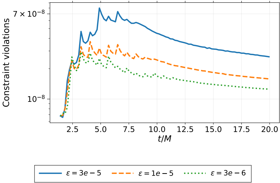
Figure 2.3 The sum of the volume weighted Hamiltonian and momentum constraint violations over the first 20M of a head-on evolution of two equal-mass charged black holes with charge-to-mass ratio q/m = 0.1 and dimensionless spin \chi = 0.4 . The simulations use wavelet tolerances of \varepsilon \in \{3 \times 10^{-5}, 1 \times 10^{-5}, 3 \times 10^{-6}\} . These simulations were done with a maximum refinement level of \ell_{\max} = 15 . Lowering the wavelet tolerance improves the resolution of dynamically important regions and reduces the overall constraint violation.
