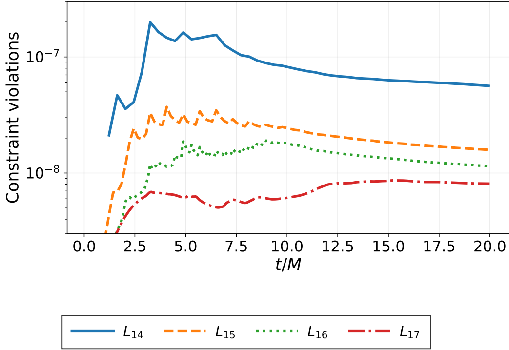
Figure E.8 The sum of the volume weighted Hamiltonian and momentum constraint violations over the first 20M of a head on evolution of two equal mass charged black holes with charge to mass ratio q/m = 0.1 and dimensionless spin \chi = 0.4 . The simulations compare maximum refinement levels j_{\max} \in \{14, 15, 16, 17\} , corresponding to finest grid spacings h \in \{0.0325, 0.0162, 0.00813, 0.00407\} , respectively. The wavelet tolerance is fixed at \varepsilon = 1 \times 10^{-5} . Increasing the maximum refinement level reduces the overall constraint violation by allowing additional grid refinement in under resolved regions.
