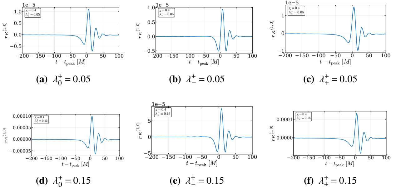
Figure I.33 Extracted axion waveforms for q = 2 and \chi = 0.4 .
