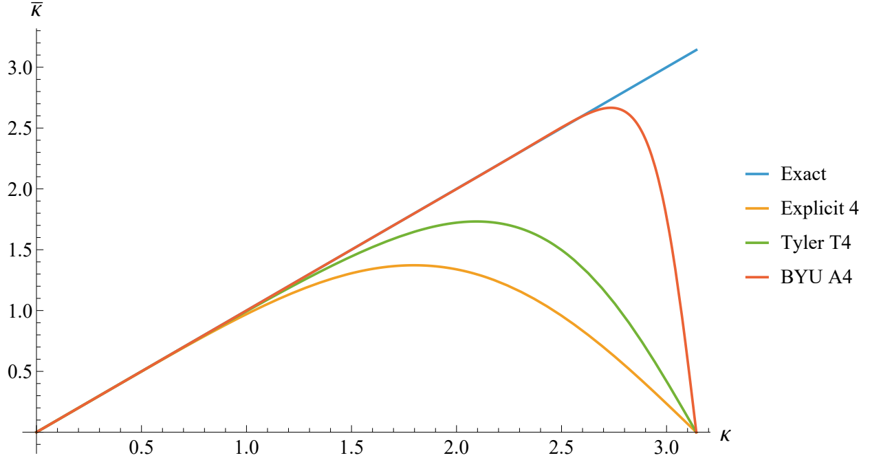
Figure 5.1 Comparison of spectral functions for several 4th order schemes: the explicit 4th order finite difference, a tridiagonal 4th order compact finite difference [ref Tyler], and a spectrally-optimized pentadiagonal 4th order compact finite difference [this work].
