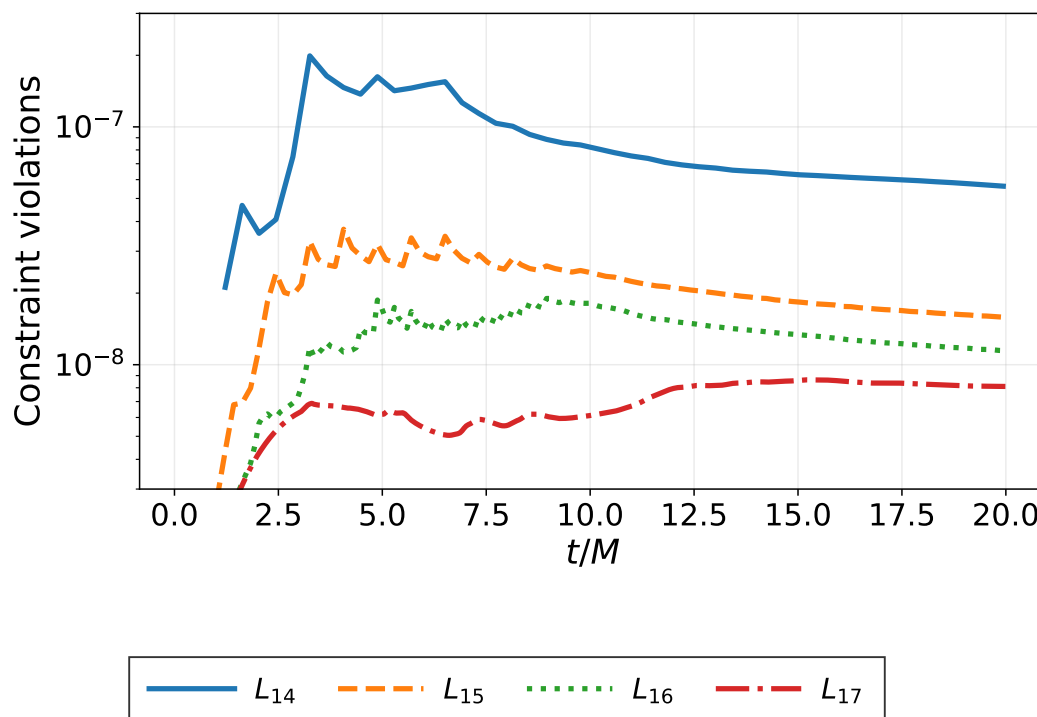
Figure 2.4 The sum of the volume weighted Hamiltonian and momentum constraint violations over the first 20M of a head-on evolution of two equal-mass charged black holes with charge-to-mass ratio q/m = 0.1 and dimensionless spin \chi = 0.4 each. The simulations compare maximum refinement levels \ell_{\max} \in \{14, 15, 16, 17\} corresponding to finest grid spacings of h \in \{0.0325, 0.0162, 0.00813, 0.00407\} , respectively. The wavelet tolerance is set here to \varepsilon = 1 \times 10^{-5} . Increasing the maximum refinement level reduces the overall constraint violation by allowing additional grid refinement in under-resolved regions.
