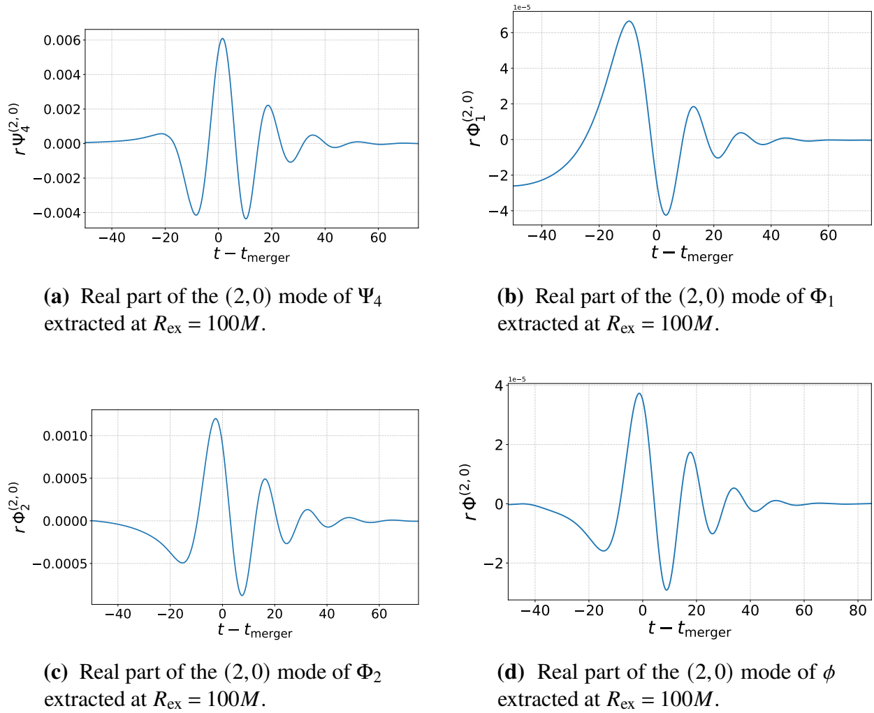
Figure 2.5 The real portions of the (2,0) modes of the gravitational radiation \Psi_4 , electromagnetic radiation \Phi_1 and \Phi_2 , and dilaton field \phi , extracted at R_{\text{ex}} = 100M for a binary with charge to mass ratio q_i/m_i = 0.1 , dimensionless spin \chi = 0.4 , and an initial coordinate separation of 16M .
