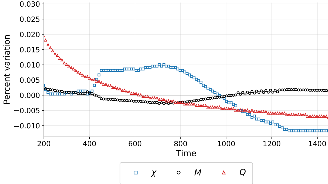
Figure 2.8 Percent deviation of the remnant black hole’s horizon mass M , electric charge Q , and dimensionless spin \chi from their calculated average values: \langle M \rangle = 0.9682 , \langle Q \rangle = 0.2001 , and \langle \chi \rangle = 0.1961 . These quantities are measured on the apparent horizon of the remnant black hole for an initially spinning and charged binary black hole configuration with individual charge to mass ratios q_i/m_i = 0.1 , initial dimensionless spins \chi = 0.4 , and total mass M = 1 .
