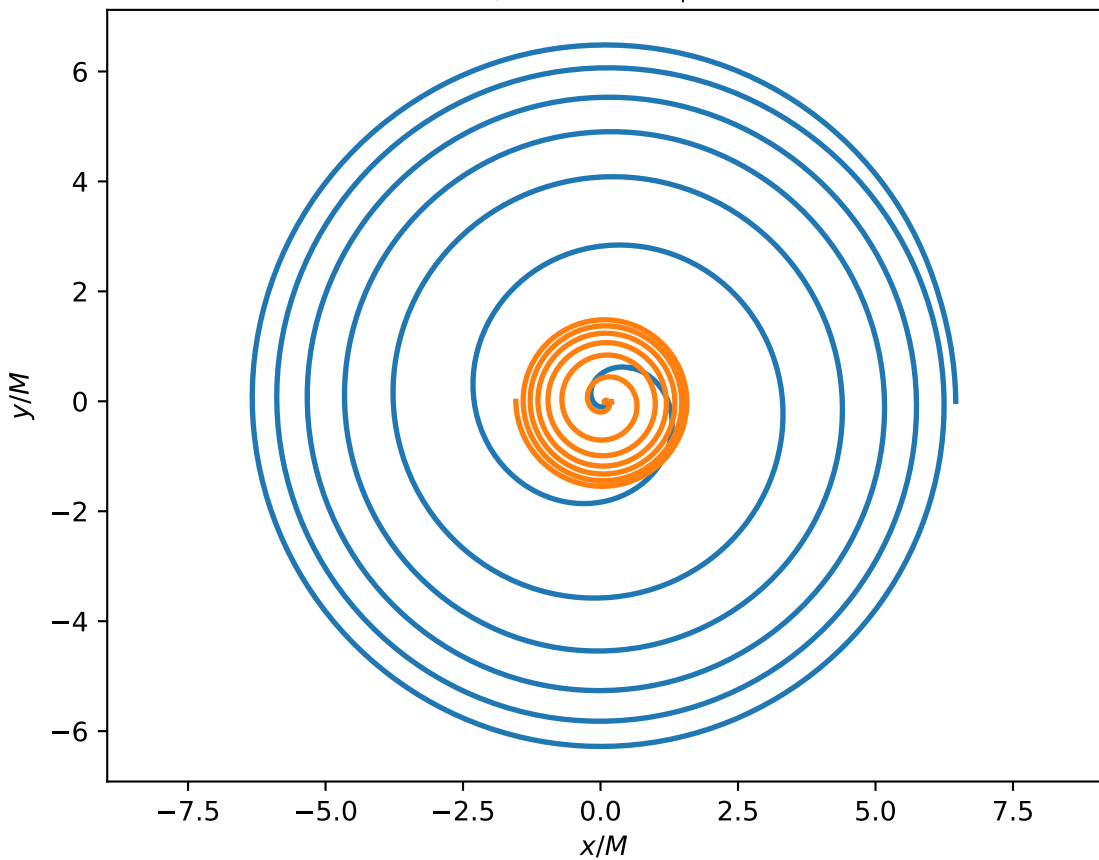
XY trajectories: \lambda_+^+ = 0.05
