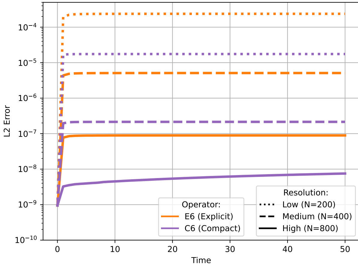
Figure 5.3 Analytic error of Burger's equation at different resolutions with 6th order operators
