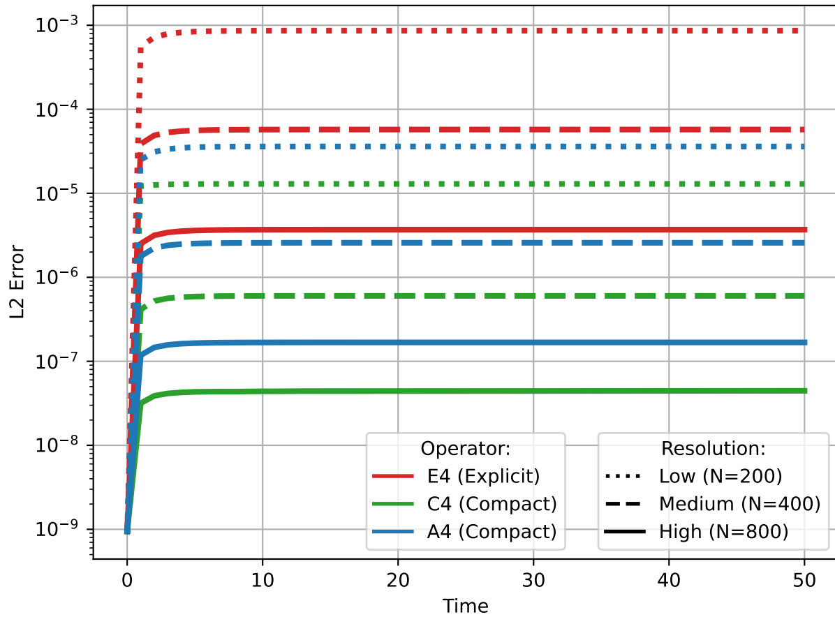
Figure 5.2 Analytic error of Burger's equation at different resolutions with 4th order operators
