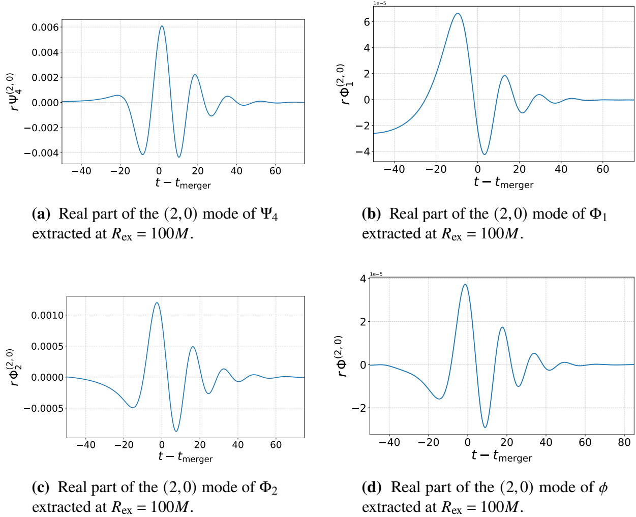
Figure 2.1 The real portions of the (2,0) modes of the gravitational radiation \Psi_4 , electromagnetic radiation \Phi_1 and \Phi_2 , and dilaton field \phi , extracted at R_{\text{ex}} = 100M for a binary with charge-to-mass ratio q_i/m_i = 0.1 , dimensionless spin \chi = 0.4 , and an initial coordinate separation of 16M .
