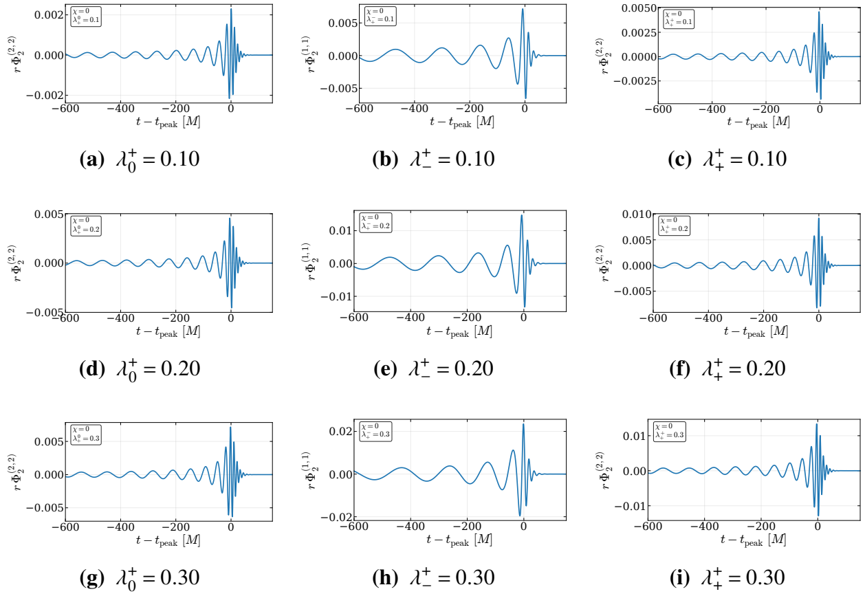
Figure H.15 Extracted \Phi_2 waveforms for q = 1 and \chi = 0 .
