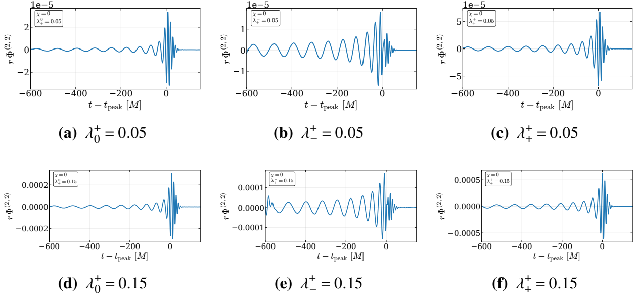
Figure H.25 Extracted dilaton waveforms for q = 2 and \chi = 0 .
