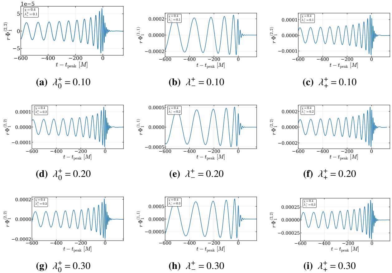
Figure H.9 Extracted \Phi_1 waveforms for q = 1 and \chi = 0.4 .
