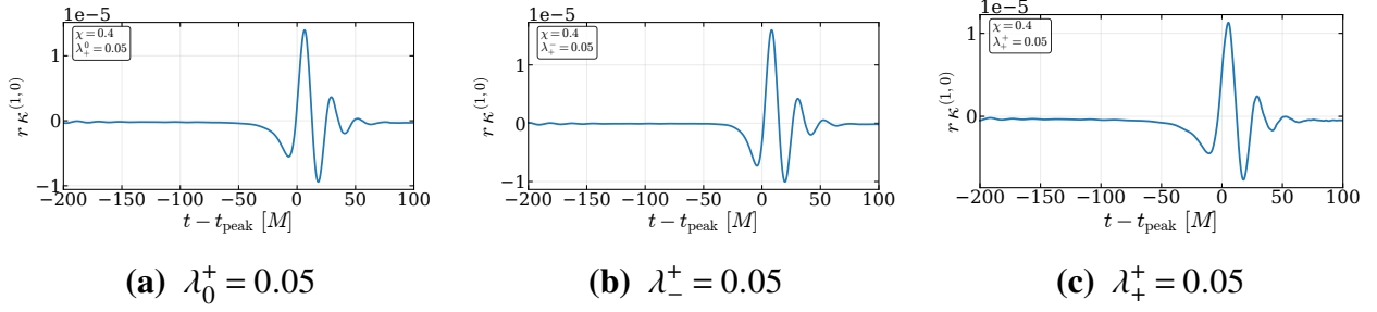
Figure H.34 Extracted axion waveforms for q = 4 and \chi = 0.4 .
