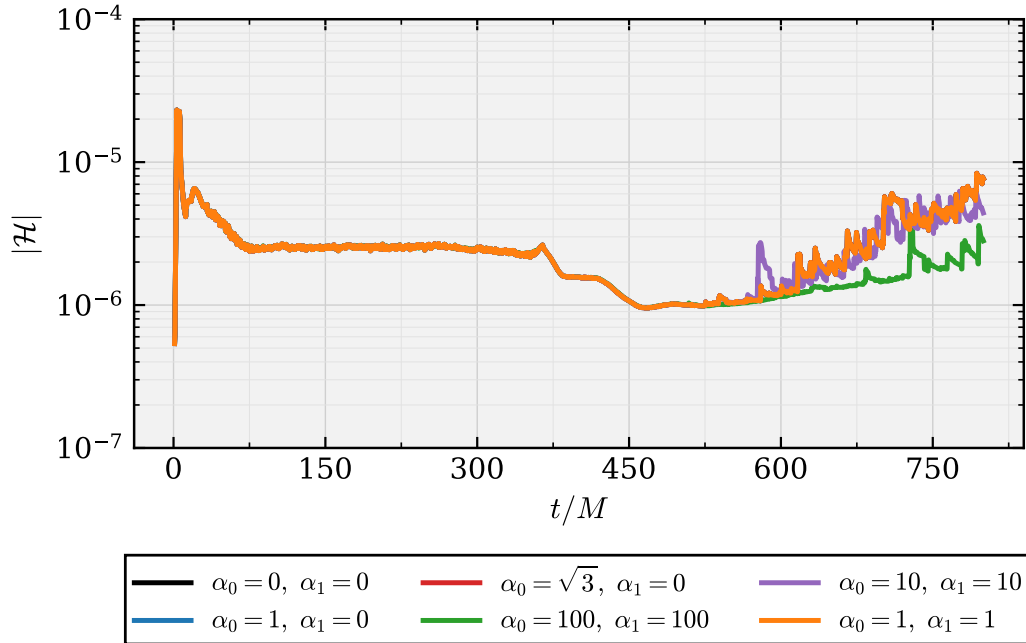
Figure 4.3 Hamiltonian constraint violation for the different coupling choices. The curves show the evolution of the Hamiltonian constraint norm for the Einstein–Maxwell reference case and the corresponding EMD and EMDA evolutions. There is an initial spike as the simulations begin, but the constraint quickly settles to a lower value. The Hamiltonian constraint does not show runaway growth and remains low throughout the evolution.
