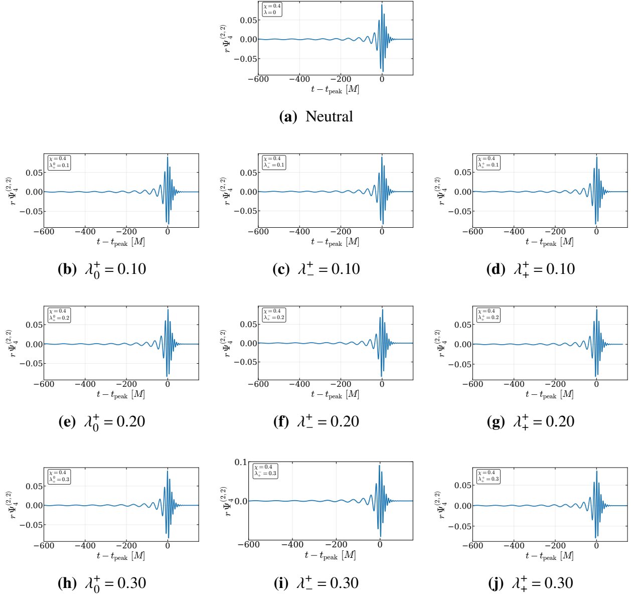
Figure H.2 Extracted r\Psi_4^{(2,2)} waveforms for q = 1 and \chi = 0.4 . The neutral case is shown at the top, followed by charged configurations ordered by increasing charge magnitude and charge configuration.
