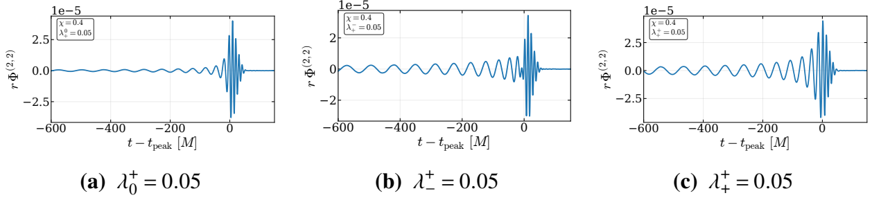
Figure H.27 Extracted dilaton waveforms for q = 4 and \chi = 0.4 .
