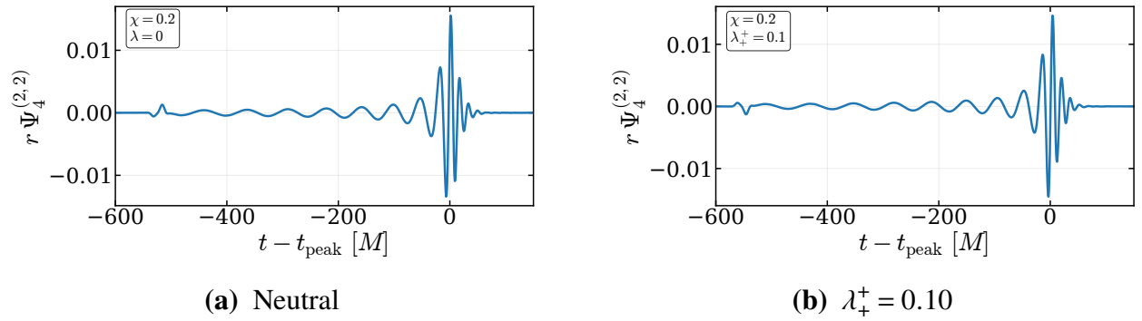
Figure H.7 Extracted r\Psi_4^{(2,2)} waveforms for q = 8 and \chi = 0.2 .
