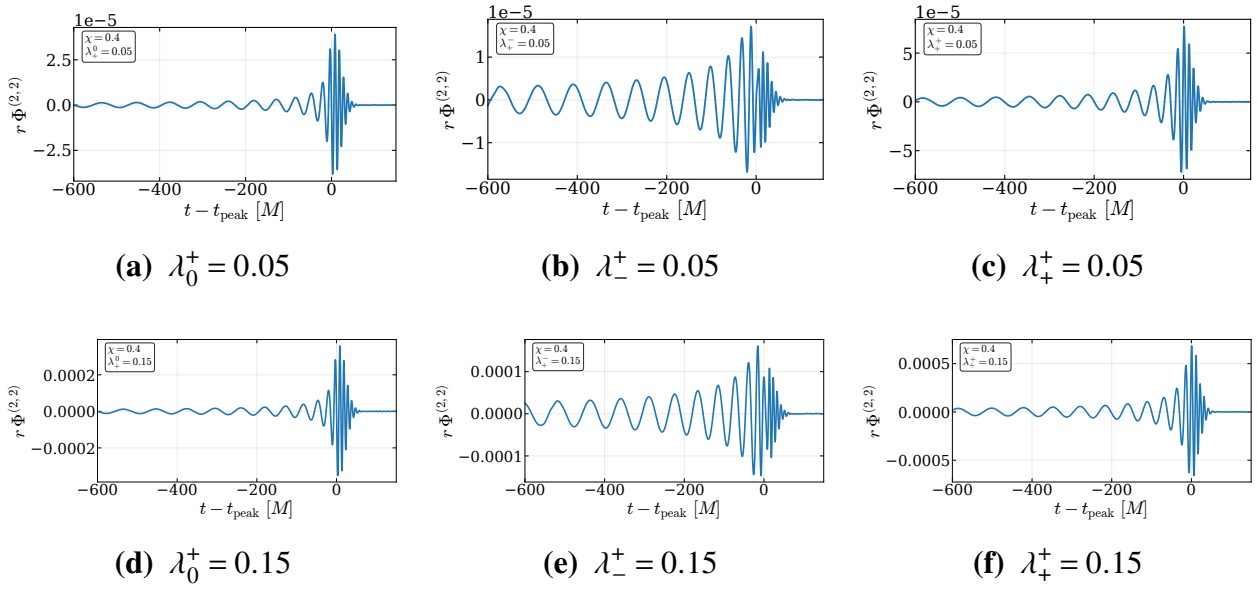
Figure H.26 Extracted dilaton waveforms for q = 2 and \chi = 0.4 .
