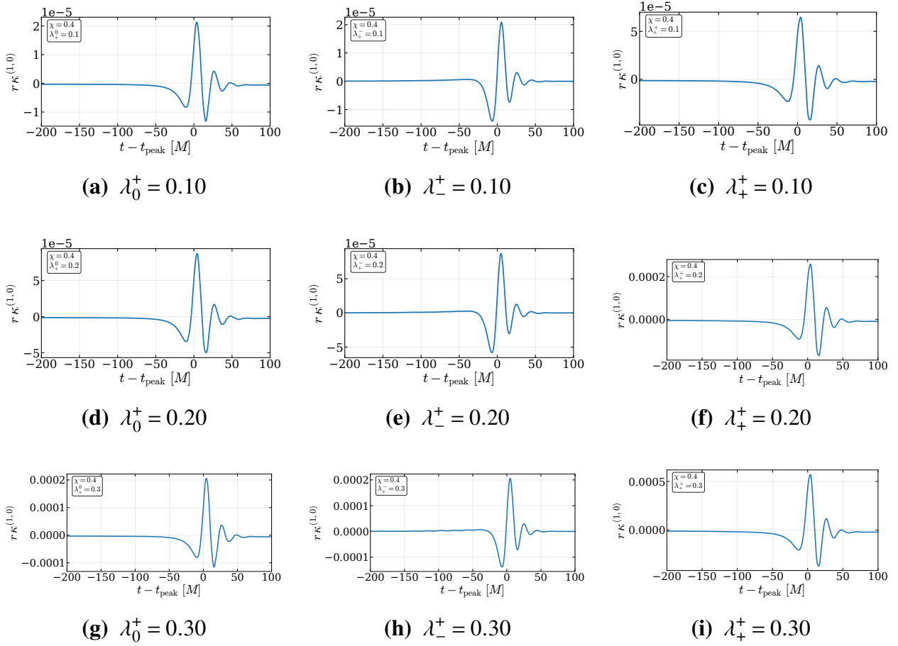
Figure H.30 Extracted axion waveforms for q = 1 and \chi = 0.4 .
