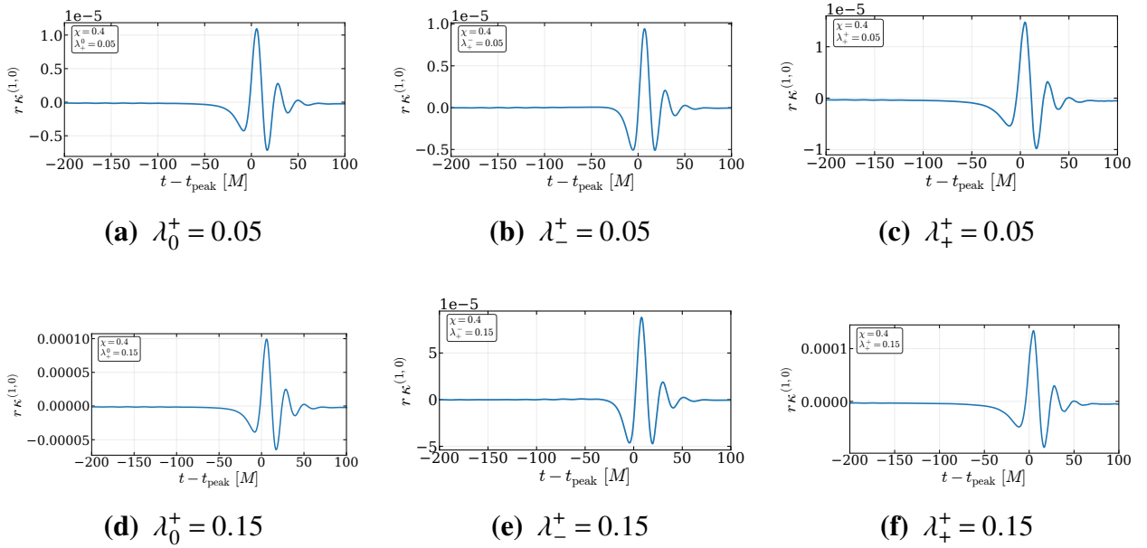
Figure H.33 Extracted axion waveforms for q = 2 and \chi = 0.4 .
