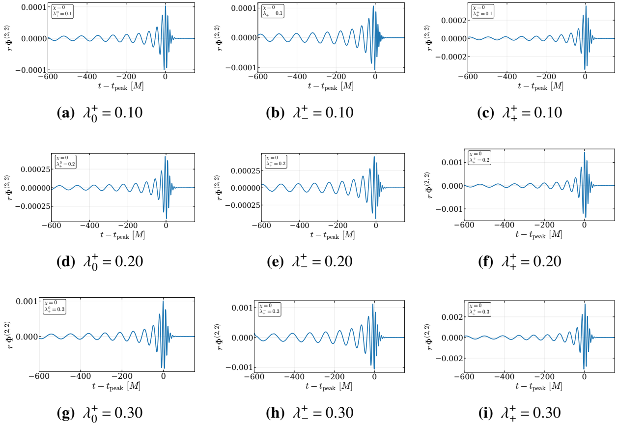
Figure H.22 Extracted dilaton waveforms for q = 1 and \chi = 0 .
