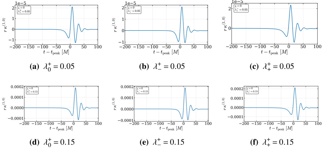
Figure H.32 Extracted axion waveforms for q = 2 and \chi = 0 .
