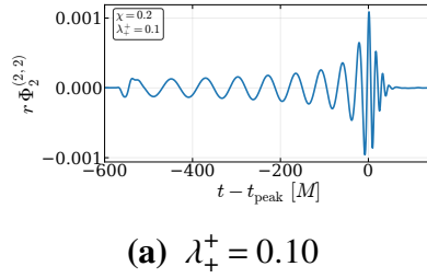
Figure H.21 Extracted \Phi_2 waveforms for q = 8 and \chi = 0.2 .
