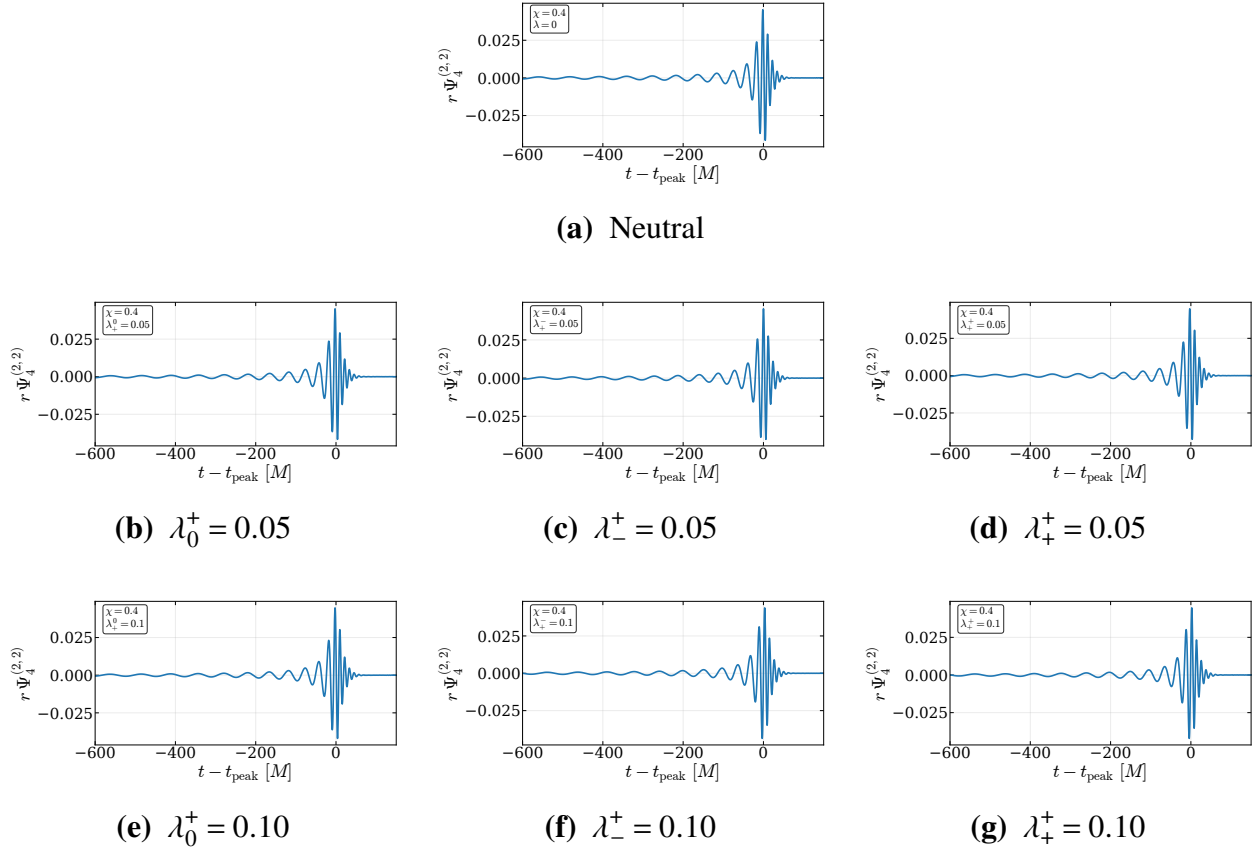
Figure H.6 Extracted r\Psi_4^{(2,2)} waveforms for q = 4 and \chi = 0.4 . The neutral case is shown at the top, followed by charged configurations with |\lambda_i| = 0.05 and |\lambda_i| = 0.10 .
