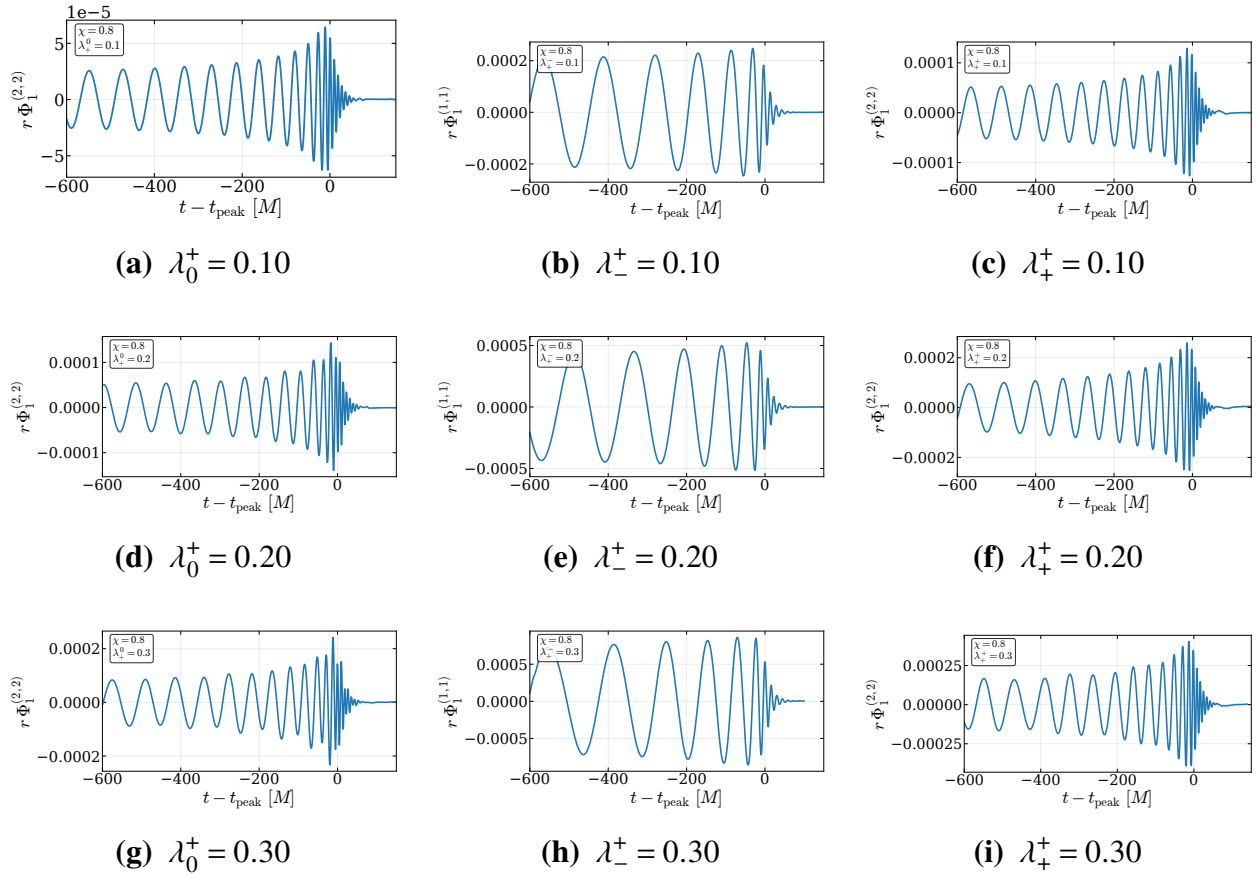
Figure H.10 Extracted \Phi_1 waveforms for q = 1 and \chi = 0.8 .
