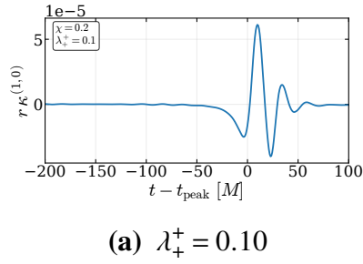
Figure H.35 Extracted axion waveform for q = 8 and \chi = 0.2 .
