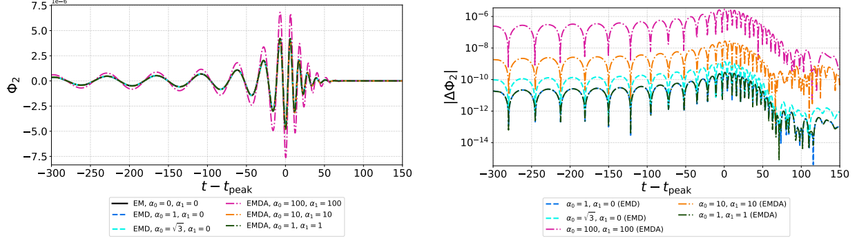
(a) Real part of \Phi_2^{22} .
