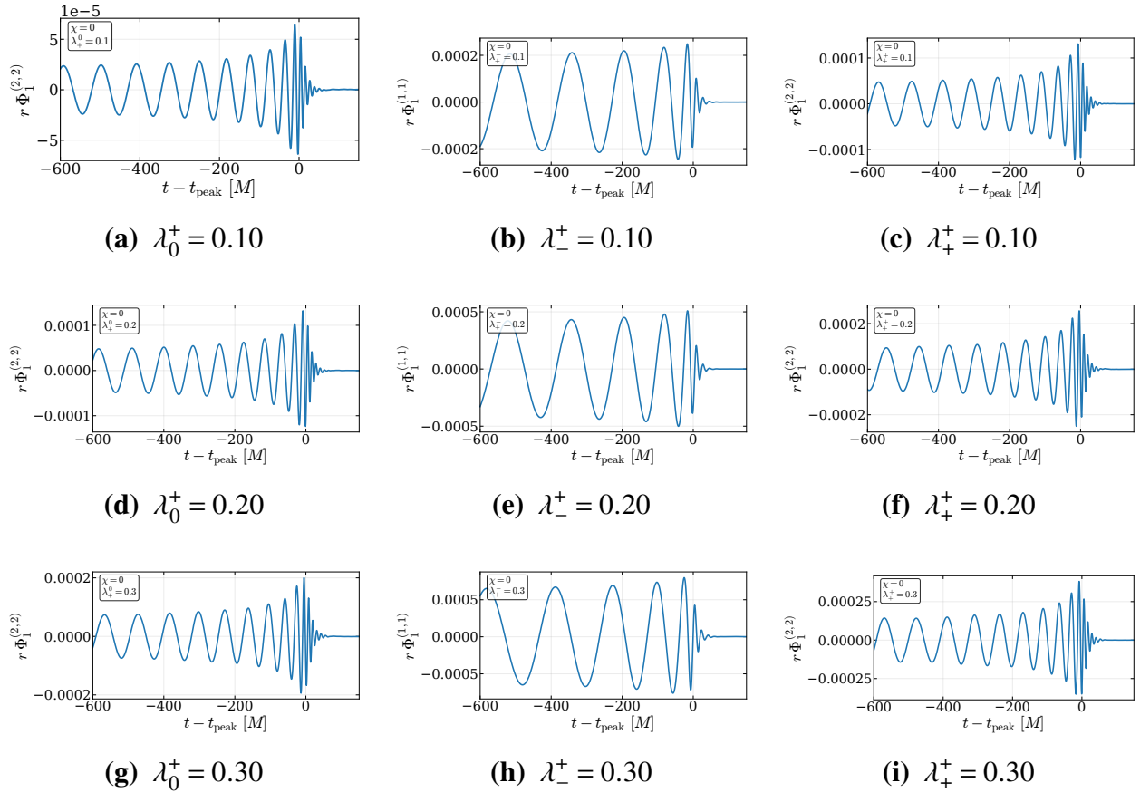
Figure H.8 Extracted \Phi_1 waveforms for q = 1 and \chi = 0 .
