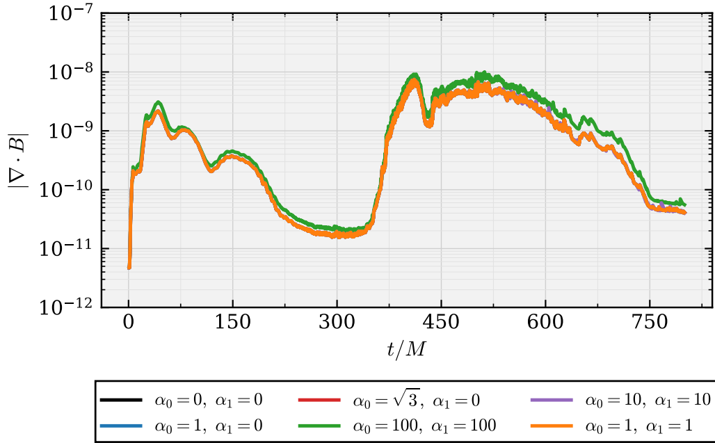
Figure 4.5 Magnetic divergence constraint violation for the different coupling choices. The curves show the evolution of the magnetic constraint norm across the Einstein–Maxwell, EMD, and EMDA evolutions. These values remain low throughout the simulation, providing confidence that the magnetic divergence constraint remains well behaved.
