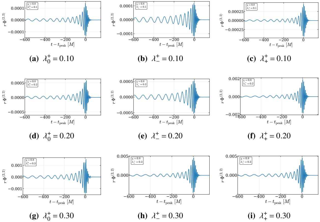
Figure H.24 Extracted dilaton waveforms for q = 1 and \chi = 0.8 .
