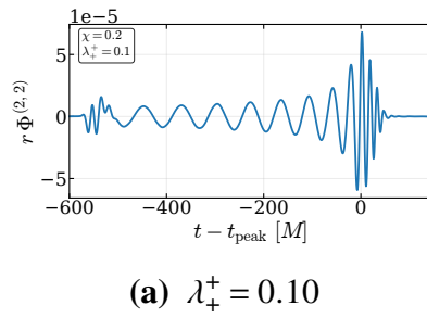
Figure H.28 Extracted dilaton waveform for q = 8 and \chi = 0.2 .
