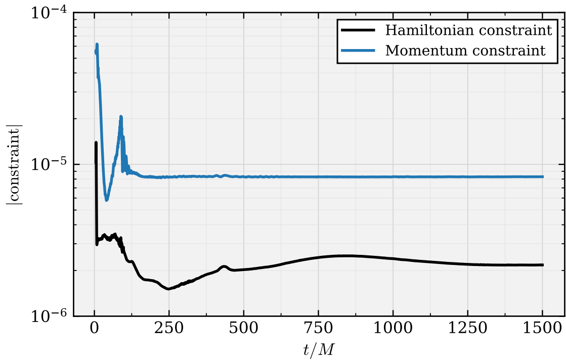
Figure E.5 The Hamiltonian constraint \mathcal{H} and the summed momentum constraint violation measured over the full simulation. The L_2 norm is normalized by the number of grid points. The constraints remain controlled throughout the evolution, including the merger phase.
