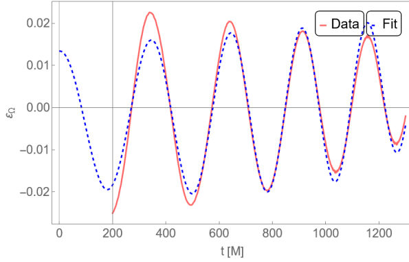
Figure 3.3 Measured (red) vs. fitted (dashed blue) orbital eccentricity for binary black hole inspiral with q = 1 , \chi = 0.4 , \lambda = 0.3 and charge configuration ++ . The data is fit from t_{\min} = 200M to t_{\max} = 1300M to avoid fitting features of the gauge wave and to fit a little bit before the ISCO (about r = 6.37M here). As reported in the table above, the measured eccentricity extrapolated to time t = 0M is \varepsilon_{\Omega} = (14.44 \pm 0.33) \times 10^{-3} .
