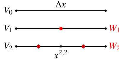
Figure E.1 Schematic illustration of nested dyadic grids used in wavelet adaptive mesh refinement. Points present on coarser grids are retained on finer grids, while the red points indicate the additional degrees of freedom introduced at each refinement level. These additional points correspond to the detail spaces W_j .
