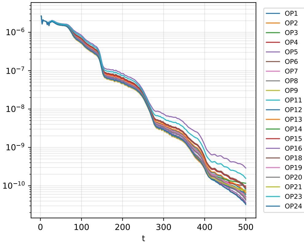
Momentum-x constraint L_2 error
