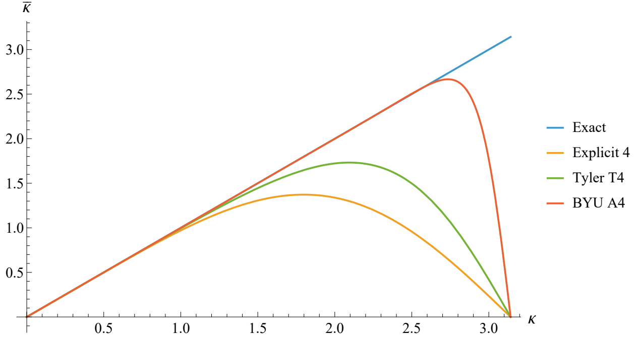
Figure 5.1 Comparison of spectral functions for several 4th order schemes. In particular, we note the explicit 4th order finite difference, a tridiagonal 4th order compact finite difference [ref Tyler], and a spectrally-optimized pentadiagonal 4th order compact finite difference [this work].
