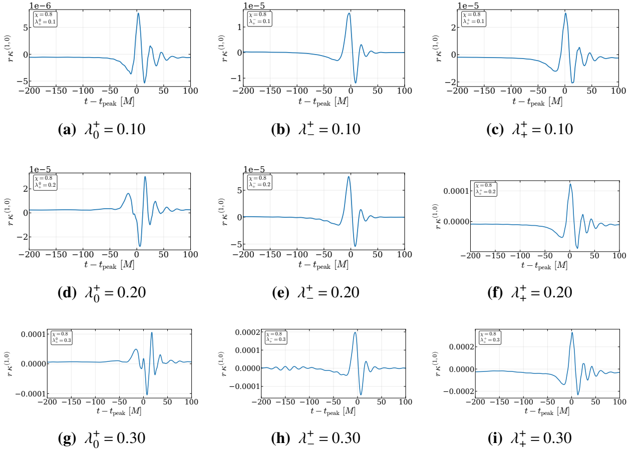
Figure I.31 Extracted axion waveforms for q = 1 and \chi = 0.8 .
