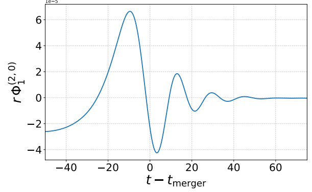
(b) Real part of the (2,0) mode of \Phi_1 extracted at R_{\text{ex}} = 100M .
