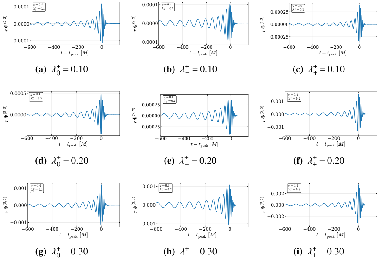
Figure I.23 Extracted dilaton waveforms for q = 1 and \chi = 0.4 .
