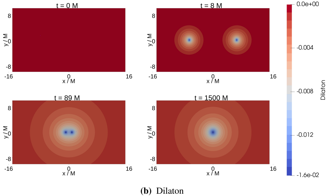
Figure 2.9 Scalar fields on the z = 0 plane for Kerr–Newman black holes with initial dimensionless spin \chi = 0.4 and charge-to-mass ratio q_i/m_i = 0.1 . Initially, neither black hole carries dilaton or axion hair. Shown are the amplitudes of the scalar fields \kappa and \phi at various stages of the evolution: the initial stage (top left), where both fields begin at zero; a short time later as the fields start to develop (top right); just before merger (bottom left); and some time after merger (bottom right).
