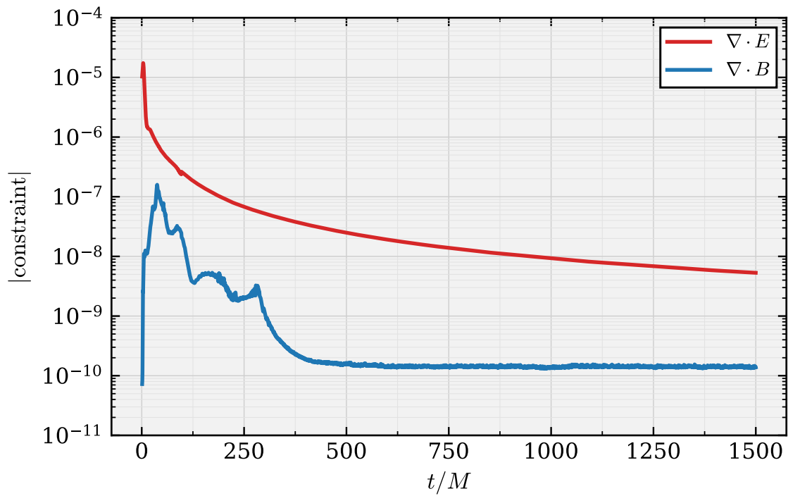
Figure 2.2 The volume weighted L_2 norms of the electromagnetic constraints measured over the full simulation. These include the magnetic no monopole constraint, \nabla \cdot B , and the electric Gauss constraint, \nabla \cdot E .
