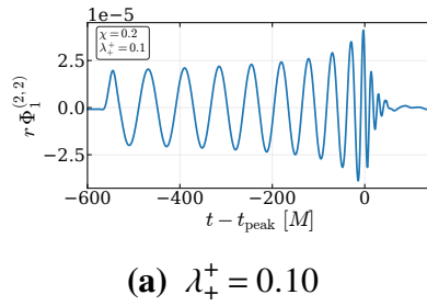
Figure I.14 Extracted \Phi_1 waveforms for q = 8 and \chi = 0.2 .
