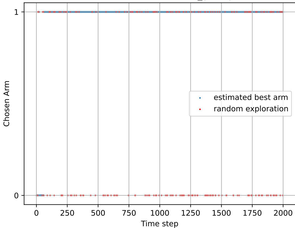
Chosen Arm over Time (e_greedy)
