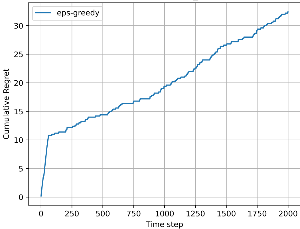
Cumulative Regret (e_greedy)
