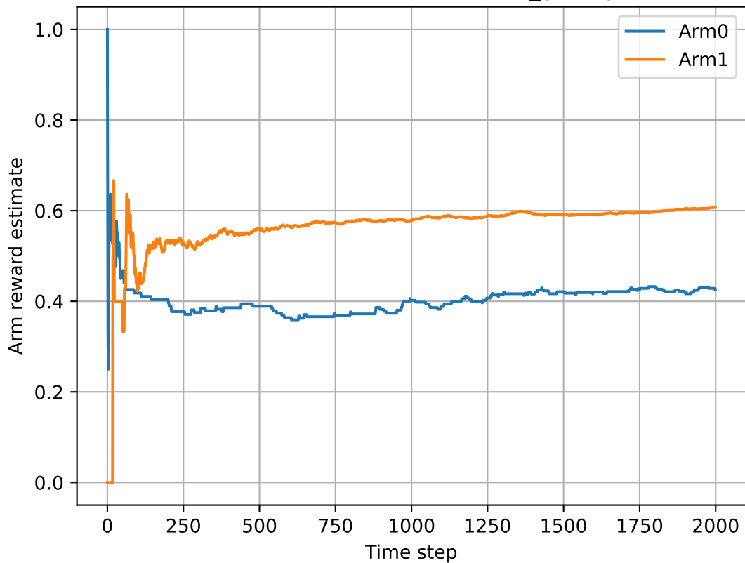
Reward estimate over time (e_greedy)
