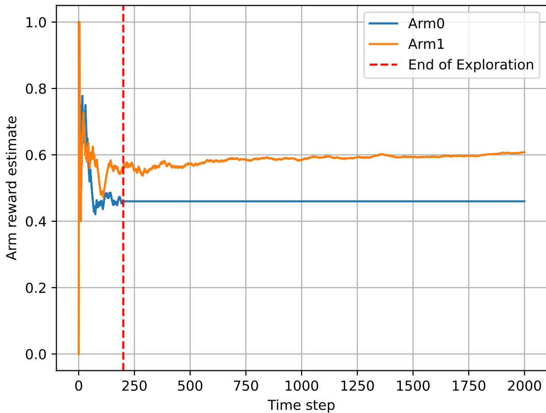
Reward estimate over time (ETC)
