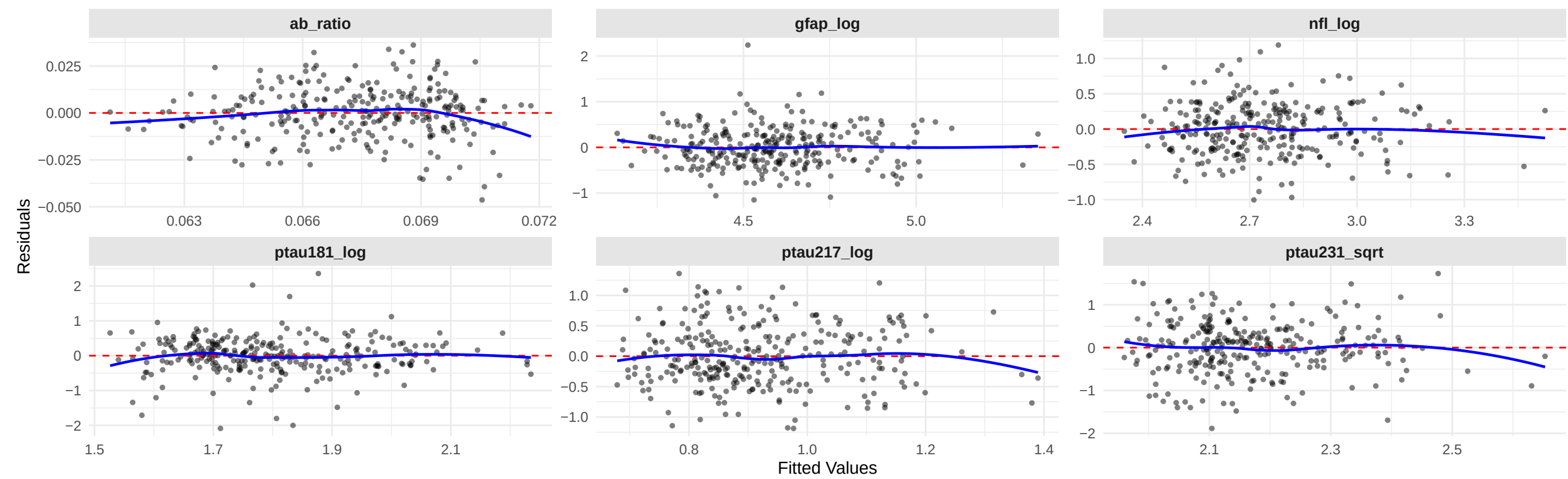
Residuals vs Fitted Values
