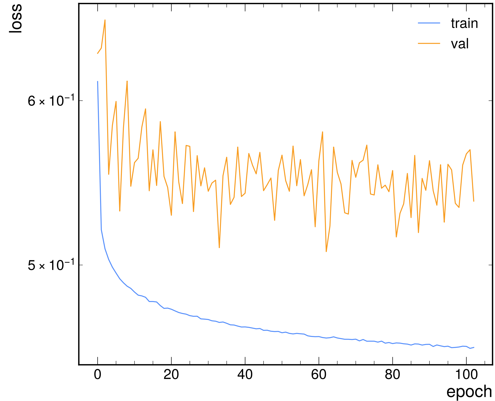
model loss
