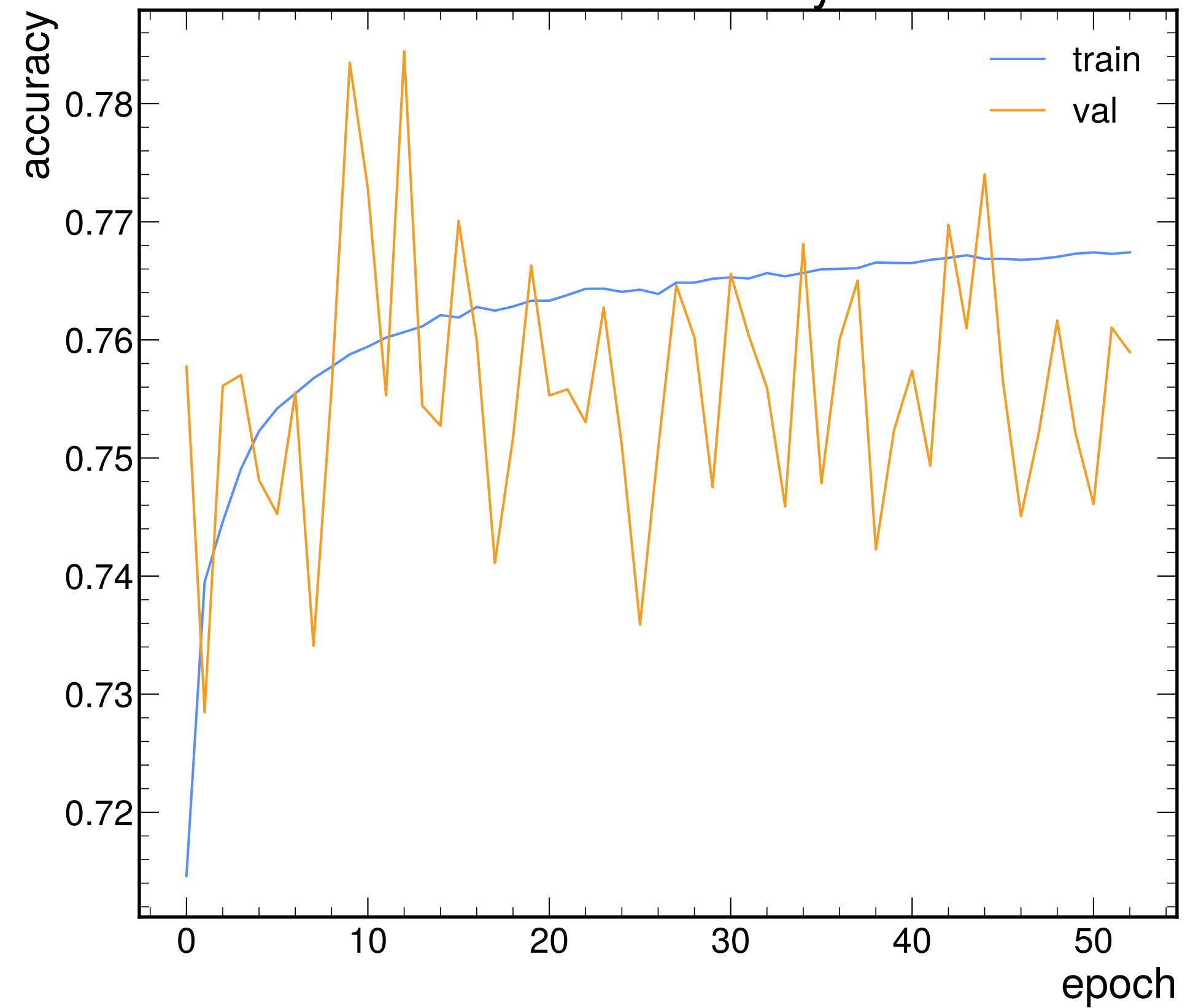
model accuracy
