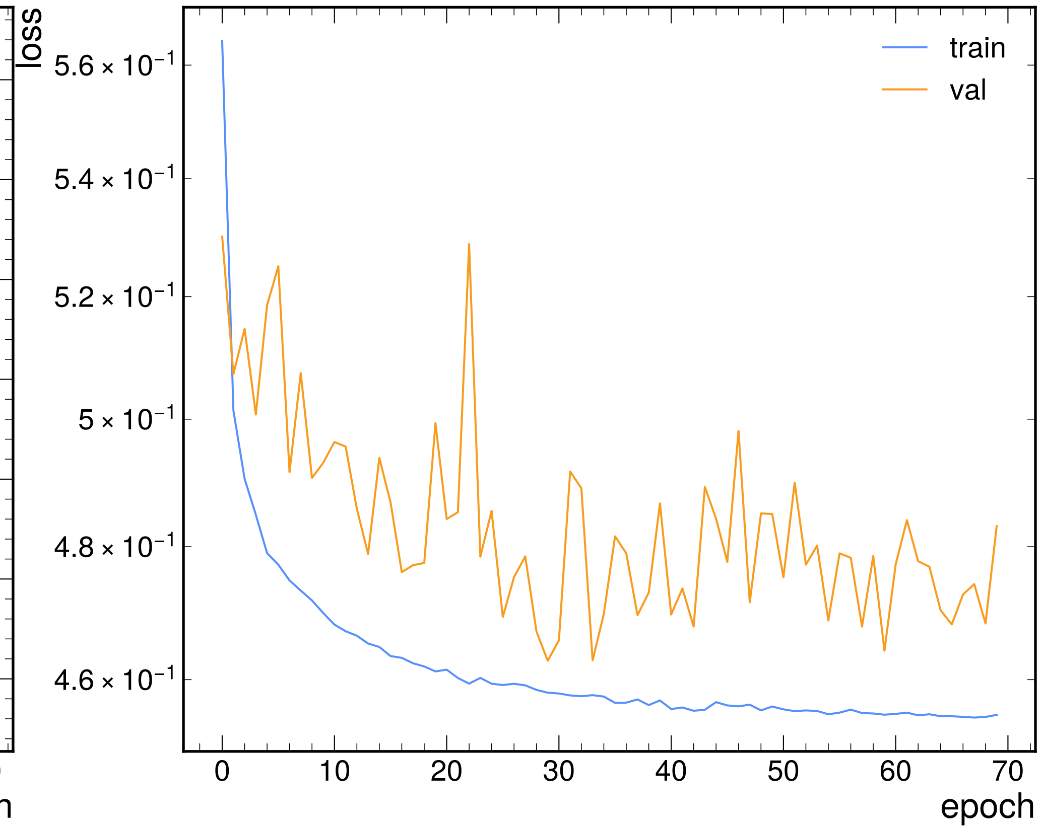
model loss
