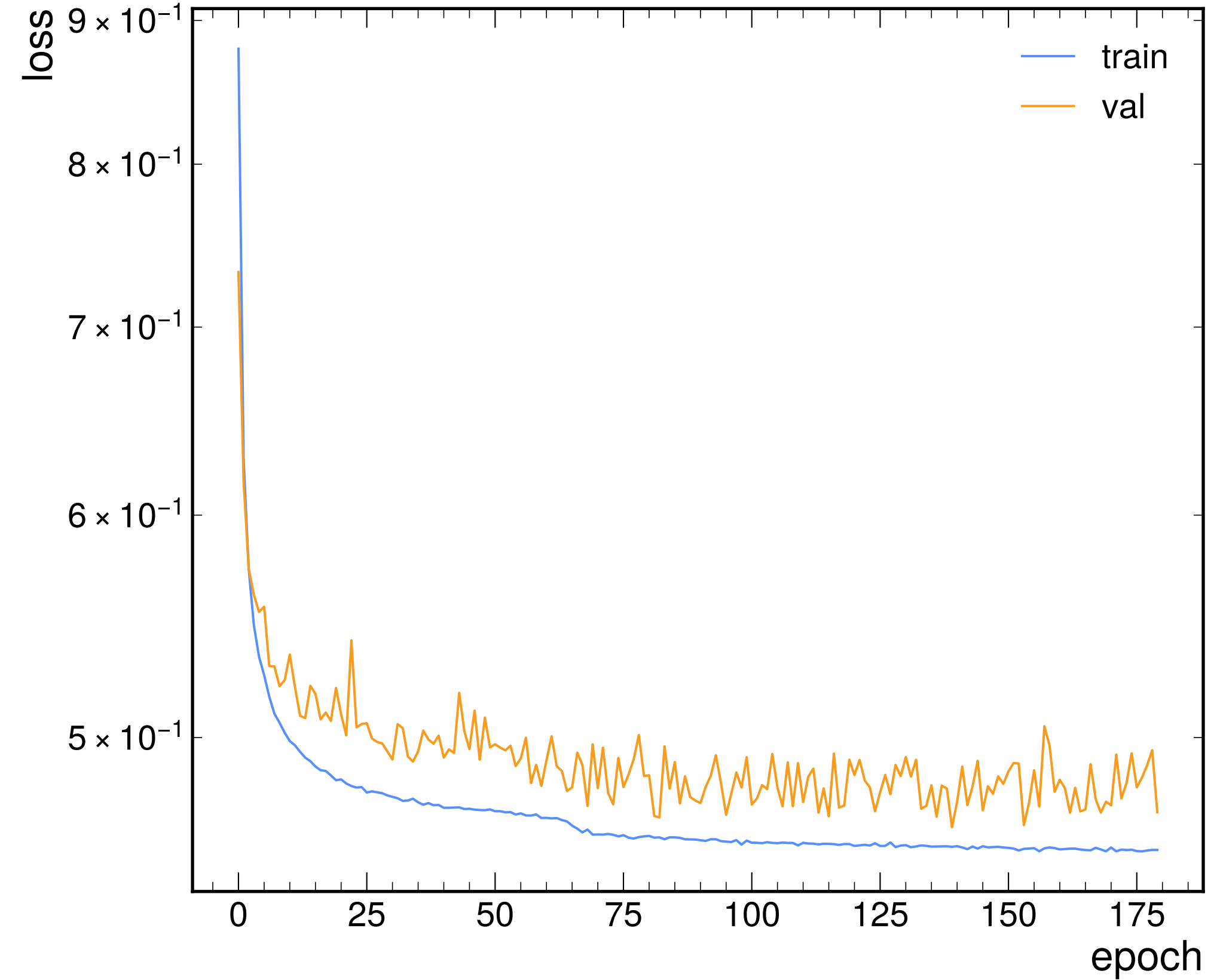
model loss
