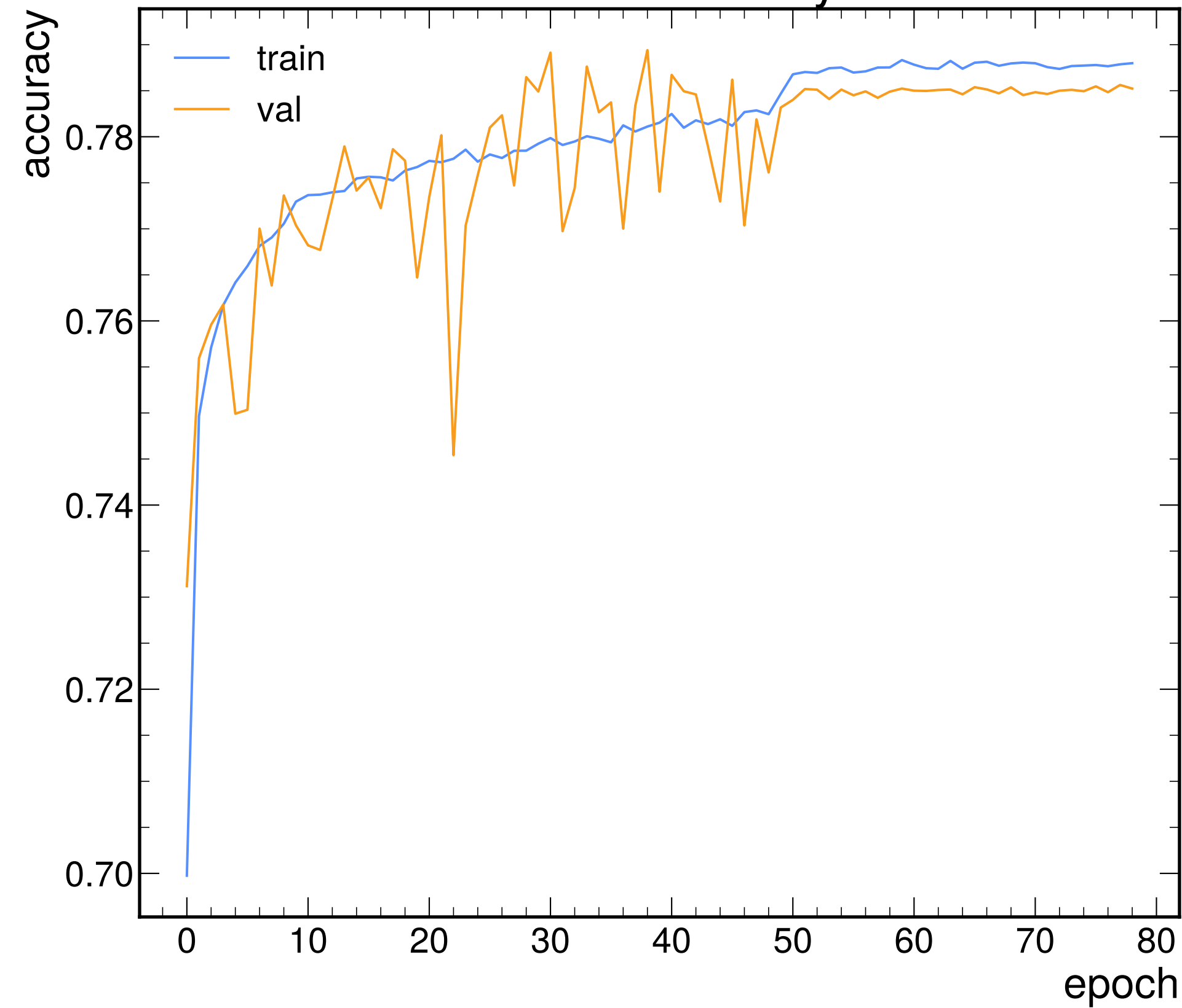
model accuracy
