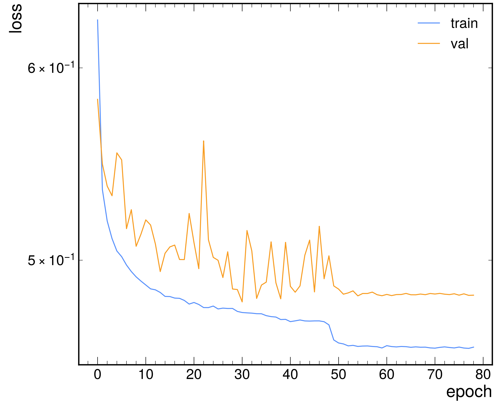
model loss
