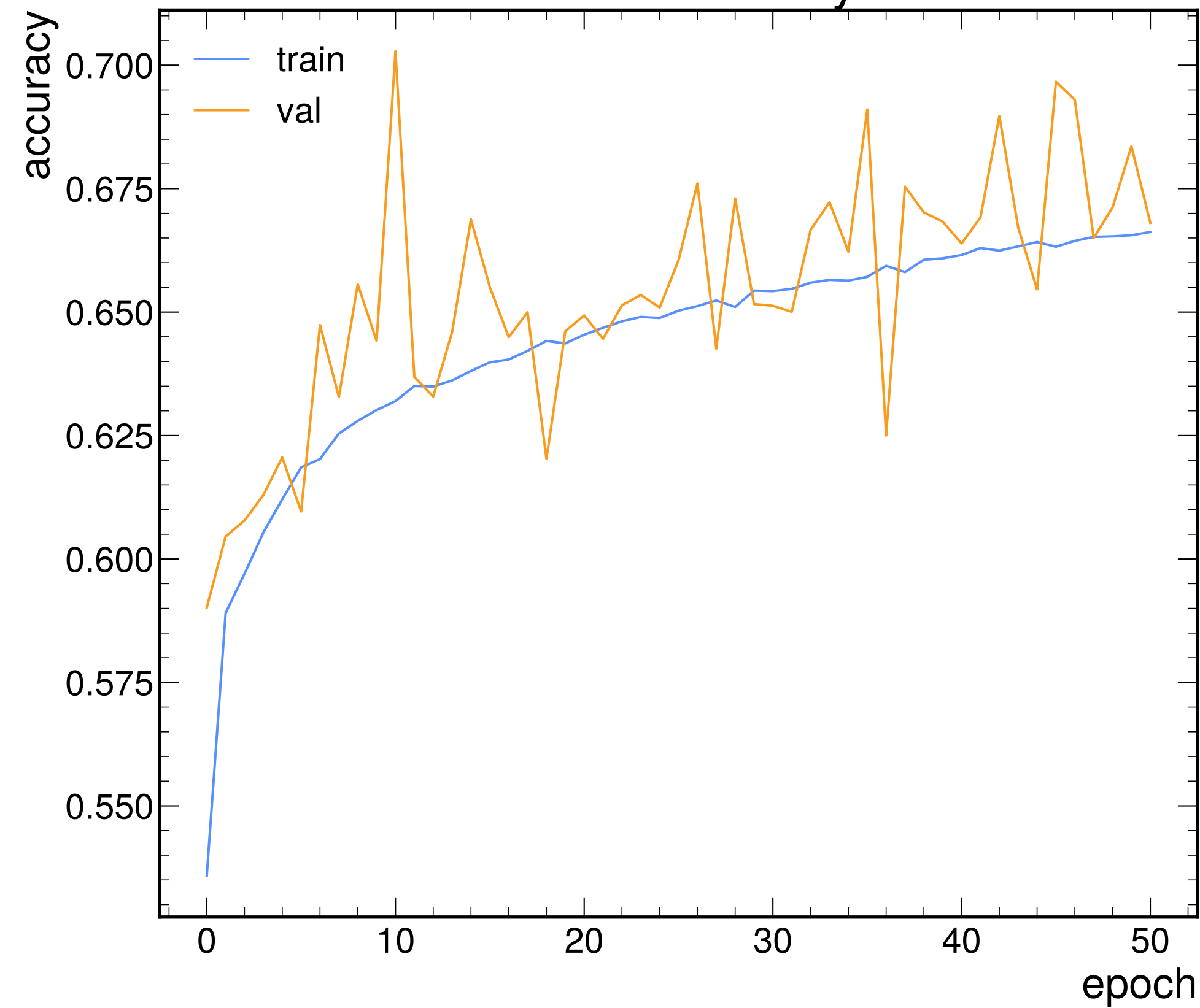
model accuracy
