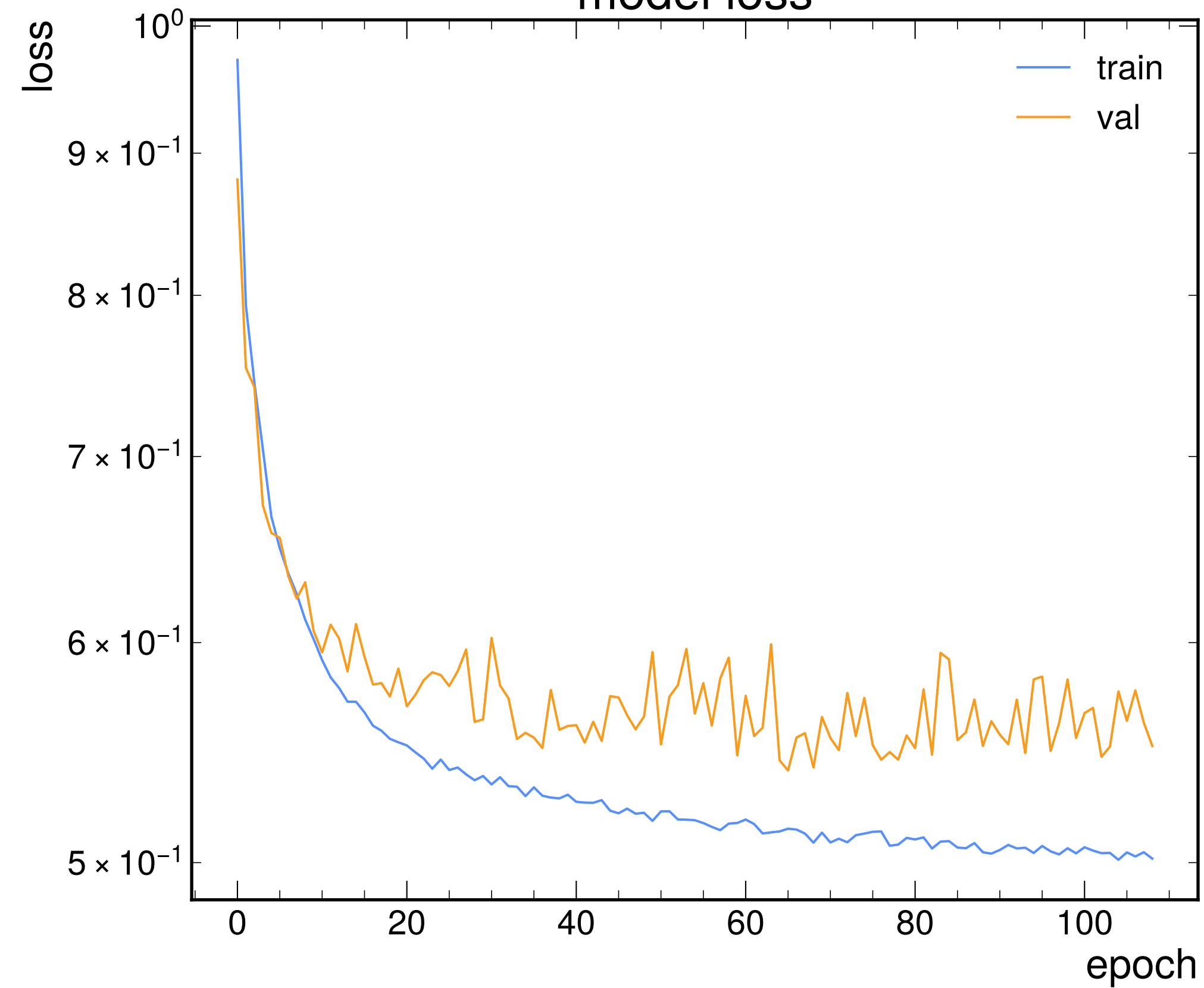
model loss
