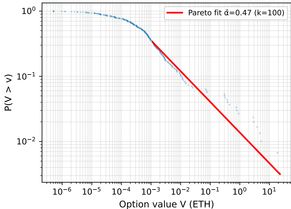
Log-log CCDF: arbitrum
