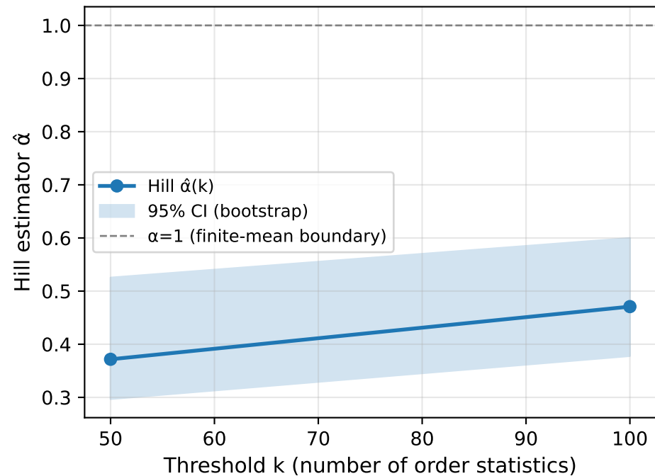
Threshold Sensitivity: arbitrum
