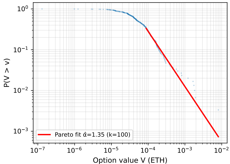
Log-log CCDF: optimism
