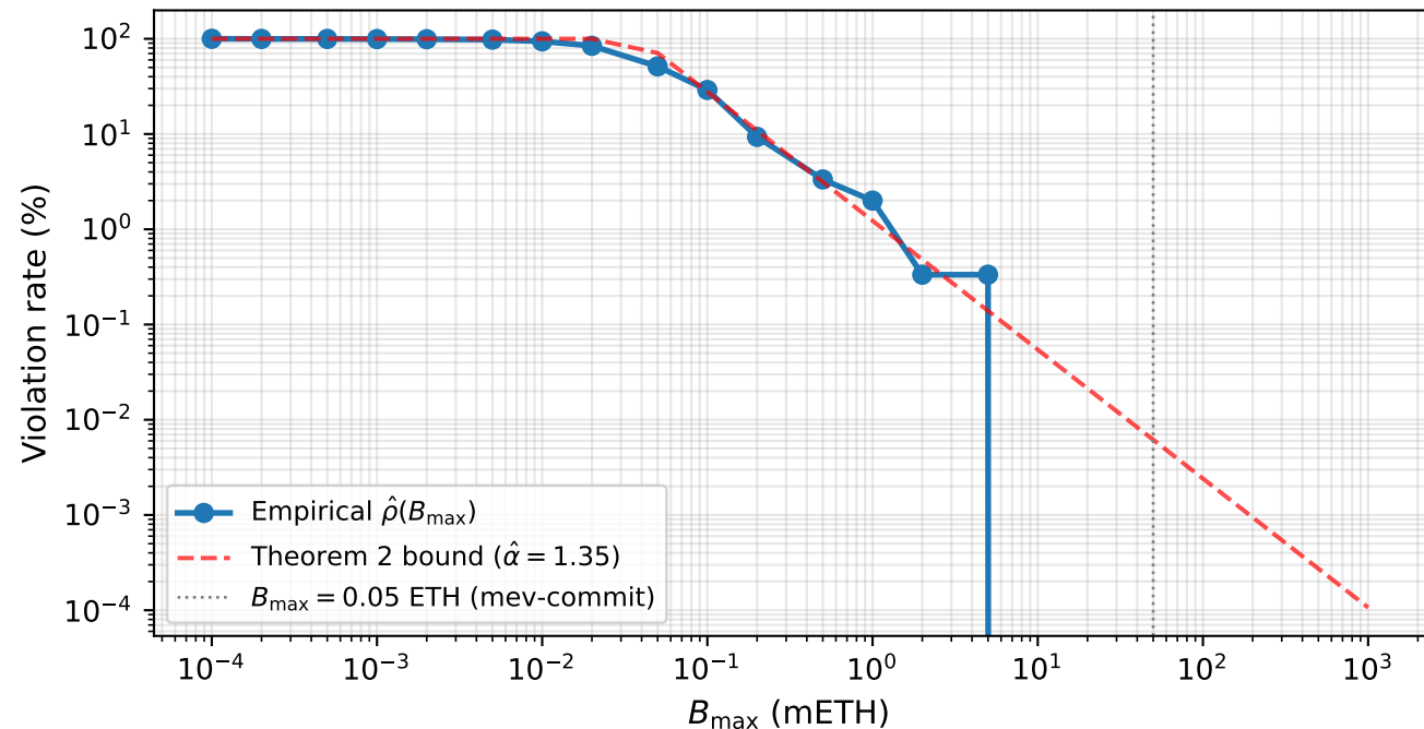
A4 Violation Rate vs. Bond: optimism
