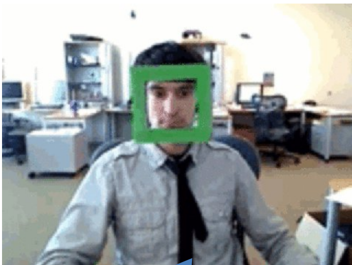
Classification + Localization
