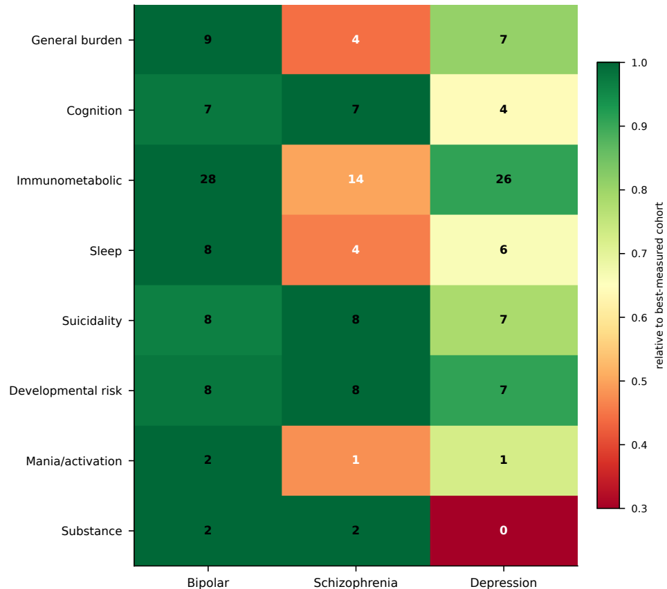
Items collected per axis (green = best-measured cohort)
