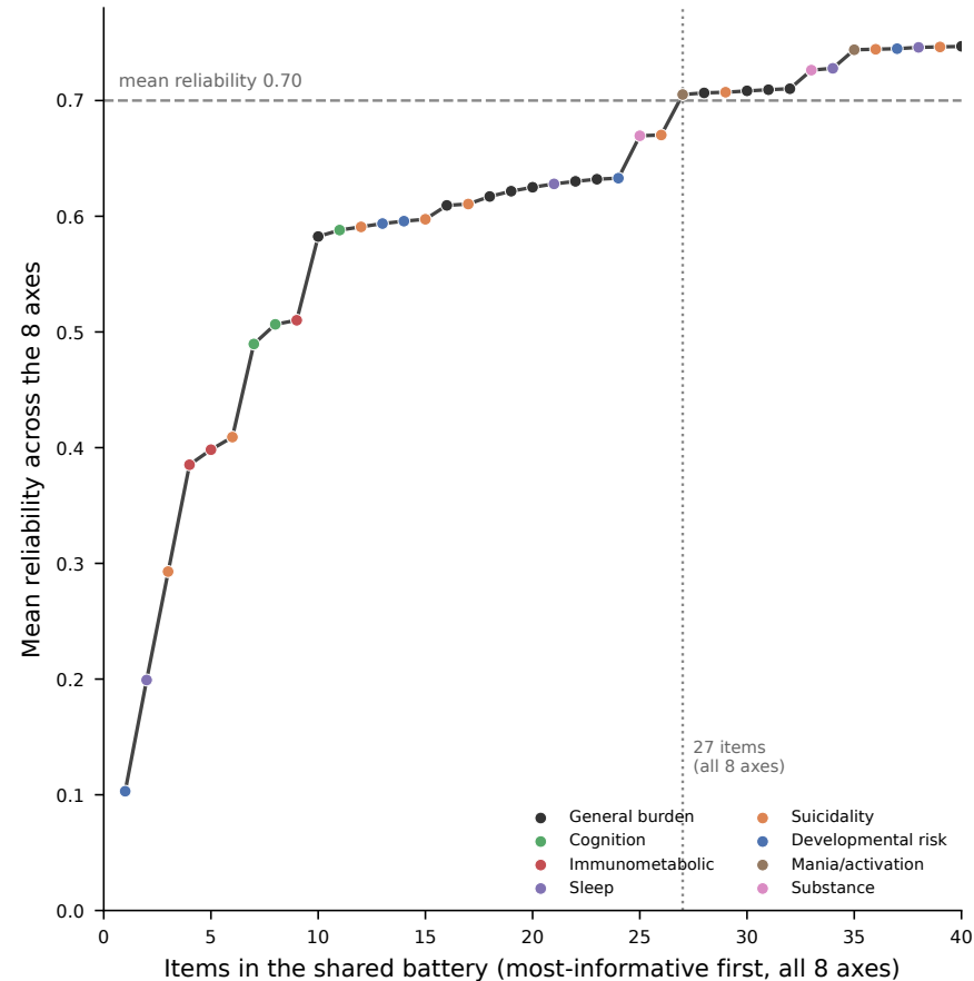
A shared 27-item battery covers all eight axes at mean reliability 0.70
