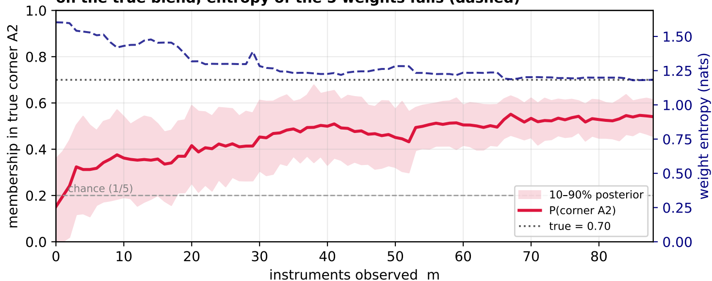
C Archotyping sharpens: membership estimate converges on the true blend; entropy of the 5 weights falls (dashed)
