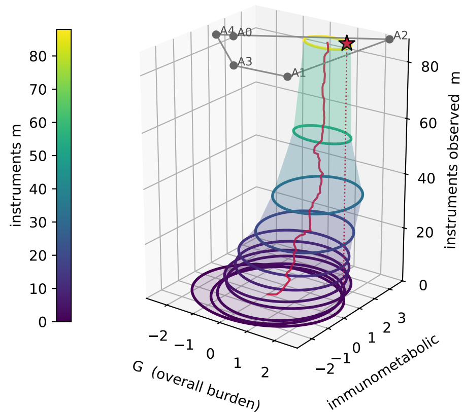
A Localization funnel: the 95% position ellipse collapses to the true patient (★, inside the A0-A4 simplex)
