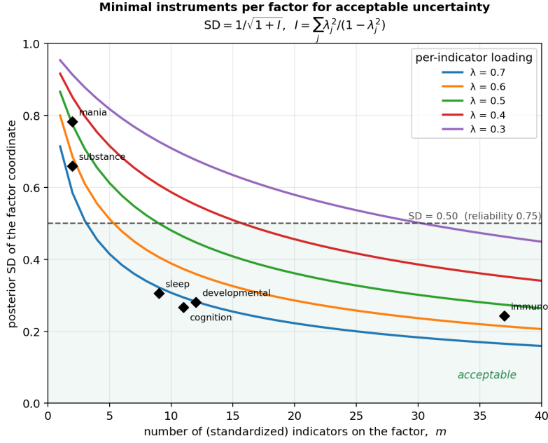
Figure 3: A minimal-indicator rule per dimension. Posterior SD of a single standardized factor coordinate against the number of indicators m , by per-indicator loading \lambda (Eq. 25). Acceptable uncertainty ( SD \leq 0.5 , reliability 0.75) needs accumulated information I \geq 3 : about 4 indicators at \lambda = 0.7 , 9 at \lambda = 0.5 , 31 at \lambda = 0.3 . Black diamonds place the FACE-ATLAS specific factors at their continuous-block indicator count and realised posterior SD; immunometabolic, developmental, cognition and sleep clear the threshold while the two-indicator mania and substance axes do not (suicidality, carried mainly by binary items, is omitted from this continuous-block illustration).
