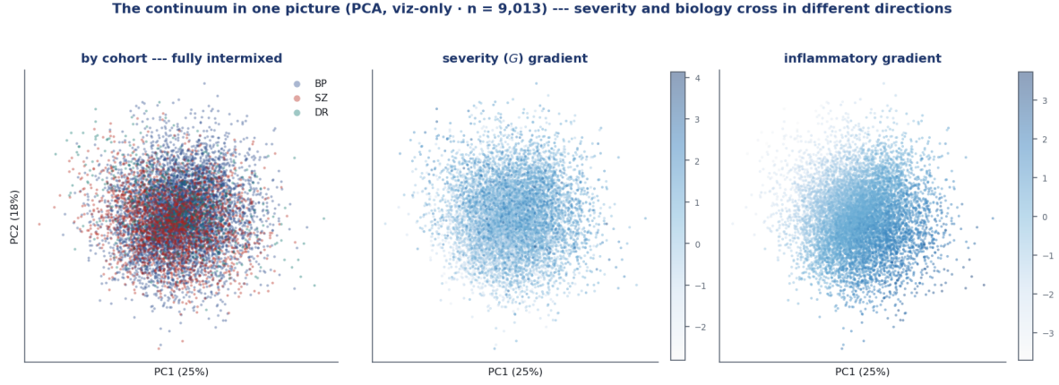
Figure 22. The continuum in one picture (PCA, visualization-only — never a clustering input). Left: by cohort — BP/SZ/DR fully intermixed, no diagnostic territories. Centre: the severity ( G ) gradient. Right: the inflammatory gradient — crossing the cloud in a different direction from severity, the geometry of biology largely independent of how impaired a patient is overall.
