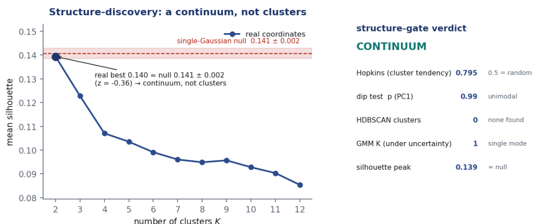
Figure 17. The falsification null. Left : silhouette by K for the real coordinates — the peak (0.140 at K=2 ) sits below the 0.15 separation floor and declines from there, so no K yields separated groups. Right : the decisive comparison — the best silhouette of the real data (0.140) lands squarely inside the distribution of best silhouettes from a single-Gaussian blob ( 0.141 \pm 0.002 , z = -0.36 ). The real cloud is statistically indistinguishable from a structureless continuum.
