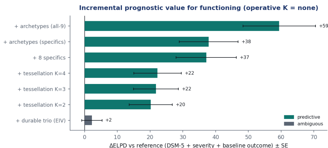
Figure 28. Incremental added value of each map encoding for two-year functioning, in held-out \Delta\text{ELPD} over the bar. The continuous/archetype encodings clear the bar by the widest margin; the hard tessellation at any K adds less and the durable trio alone is ambiguous — the visual form of the operative- K = \text{none} verdict.
