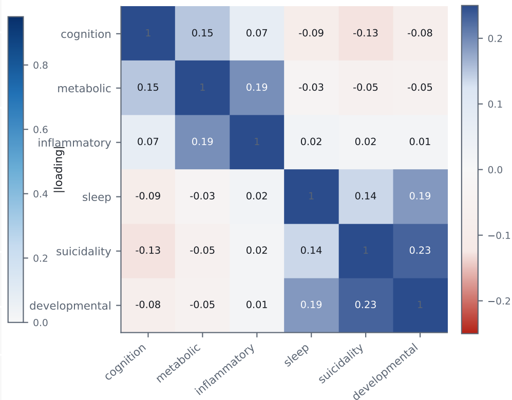
b Inter-dimension correlations \Phi
