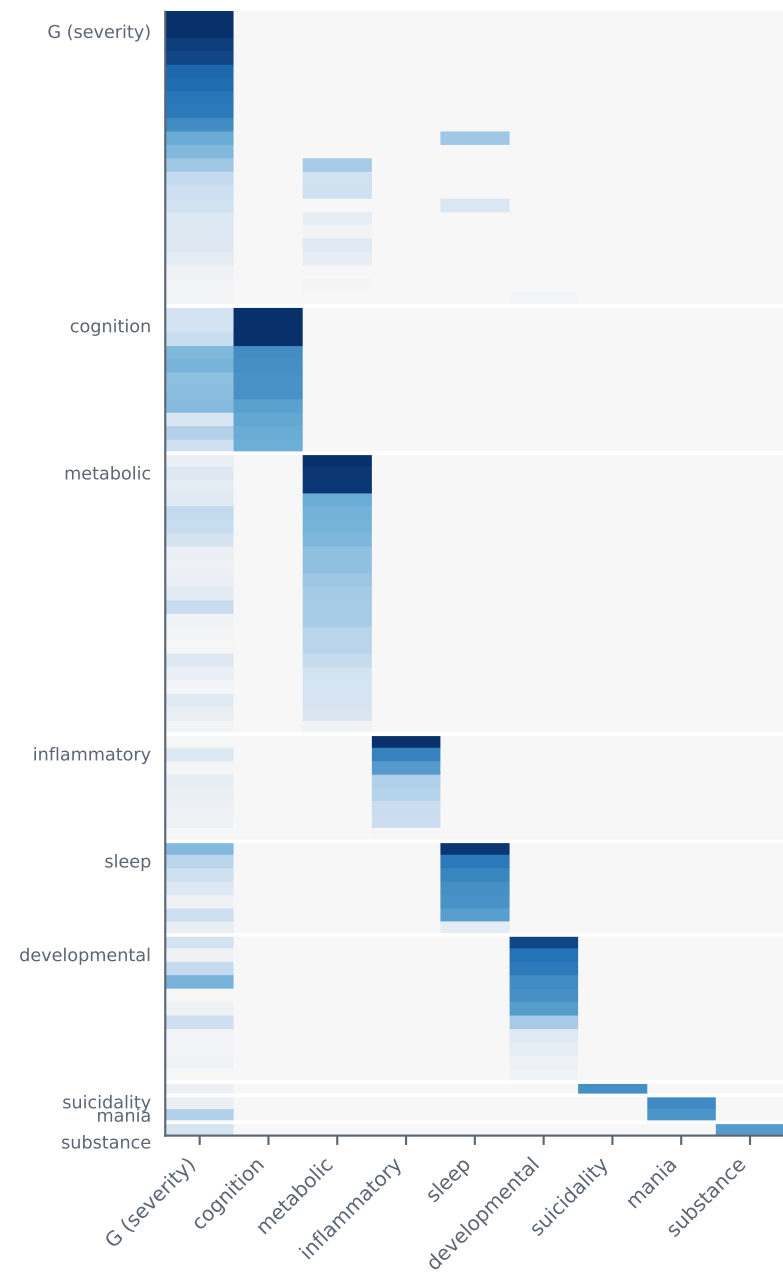
a Posterior loading atlas (the data)
